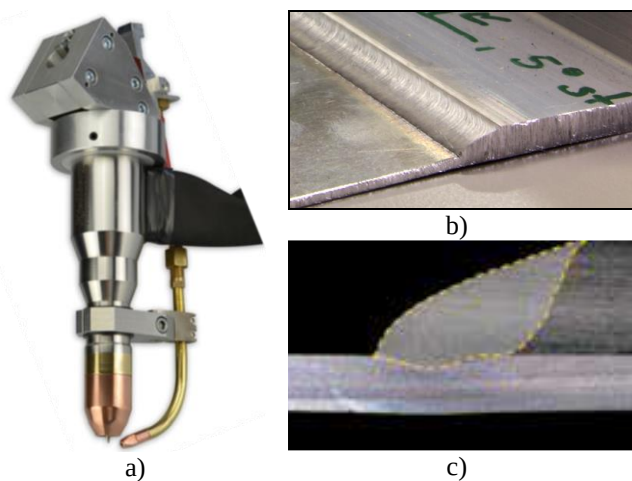
Figure 3. Equipment for plasma welding: a) Kjellberg welding head; b) layer-by-layer welding of the product; c) welding section (information from www.kjellberg.de )
