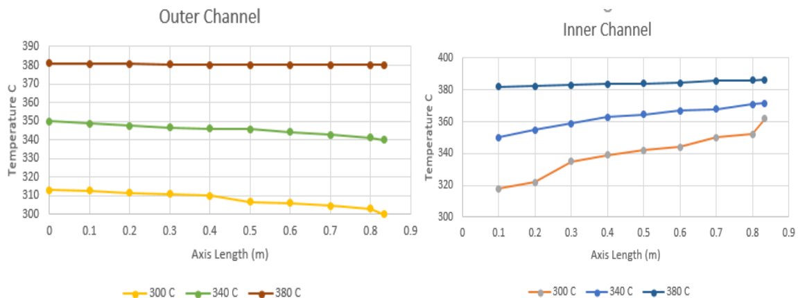
Figure 1 - Dependence of the coolant temperature at 300°C, 340°C, 380°C on the channel length
