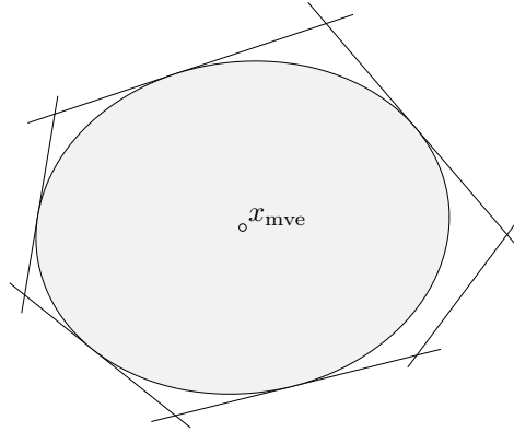
Figure 8.6 The lightly shaded ellipsoid shows the maximum volume ellipsoid contained in the set C , which is the same polyhedron as in figure 8.5. Its center x_{mve} is the maximum volume ellipsoid center of C .
