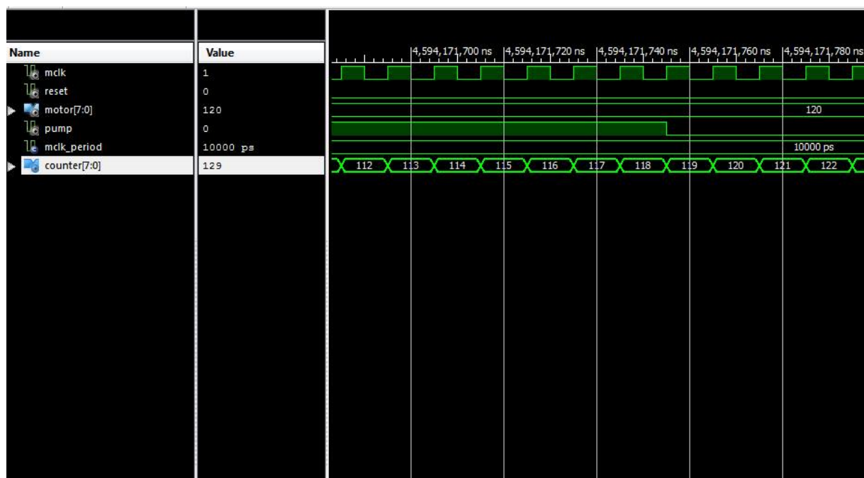
Figure 4. Operation of the pump.
