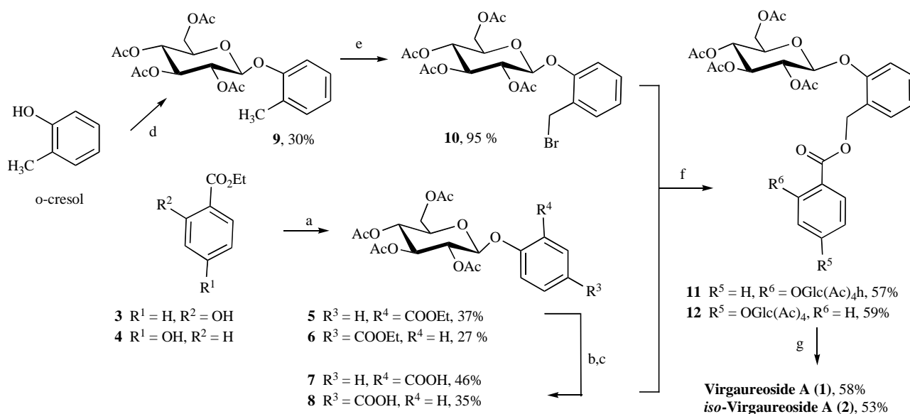
Fig. (1). Structures of Virgaureoside A and iso-Virgaureoside A.
