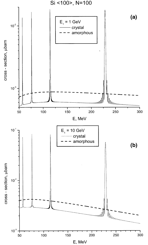
Fig. 3. The cross-section of coherent type B production of Ps by relativistic electrons as a function of created Ps energy for two electron energies E_1 = 1 GeV (Fig. 4(a)) and E_1 = 10 GeV (Fig. 4(b)). Dashed lines show the cross-section of the Ps production by electrons in an amorphous target of equivalent thickness, which contains the same number N of atoms as a crystal. The maximal emission angle of Ps is \Theta_m = 5 mrad. The parameters of the crystal are the same as in Fig. 1.
