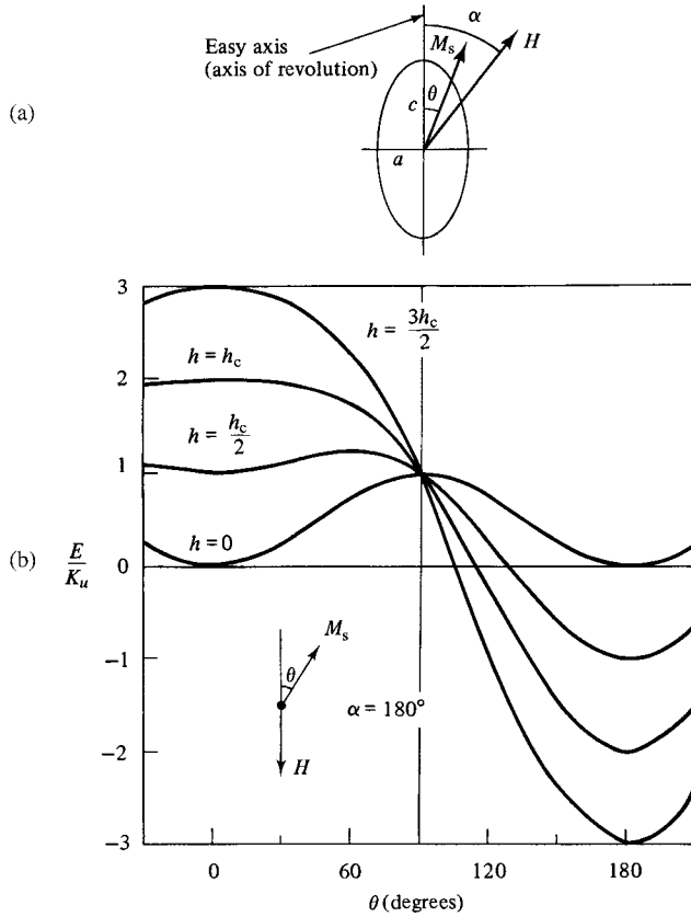
Fig. 9.35 Rotation of magnetization by a field applied to a single-domain ellipsoid; h is a reduced field H/H_K (see text).
