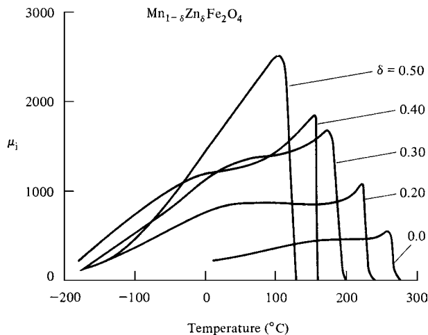
Fig. 13.27 Variation with temperature of the initial permeability \mu_i of Mn-Zn ferrites. These specimens also contain a small ferrous ( \text{Fe}^{2+} ) ion content.
