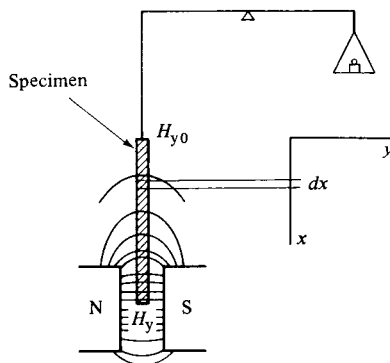
Fig. 2.48 Gouy method for measurement of susceptibility.
