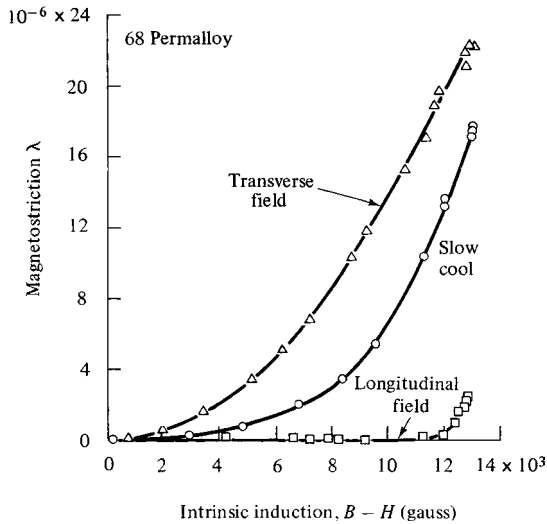
Fig. 10.3 Magnetostriction of a 68 Ni–32 Fe alloy after various treatments. [H. J. Williams et al. Phys. Rev. , 59 (1941) p. 1005.]
