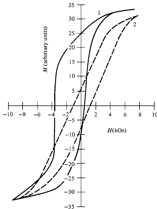
Fig. 11.25 Hysteresis loops measured at 77K of oxide-coated cobalt particles. Loop (1) results from cooling in a 10 kOe field in the positive direction, and loop (2) from cooling in zero field. [W. H. Meiklejohn and C. P. Bean, Phys. Rev. , 105 (1957) p. 904.]
