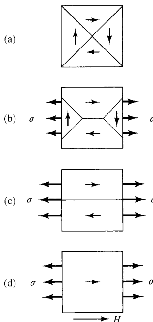
Fig. 8.21 Magnetization of a material with positive magnetostriction under tensile stress (schematic).
