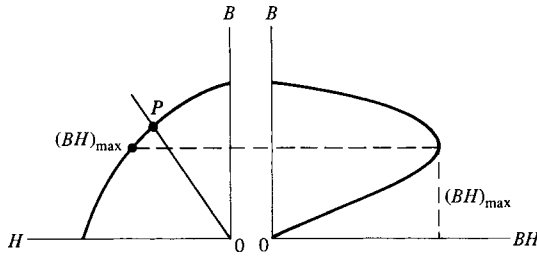
Fig. 14.3 Left: demagnetization curve; right: corresponding values of energy product ( BH ) plotted on the same B scale. Maximum value of ( BH ) is shown on both plots.
