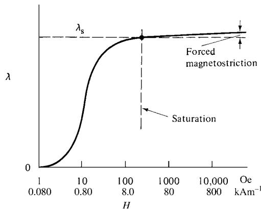
Fig. 8.1 Dependence of magnetostriction on magnetic field (schematic). Note that the field scale is logarithmic.
