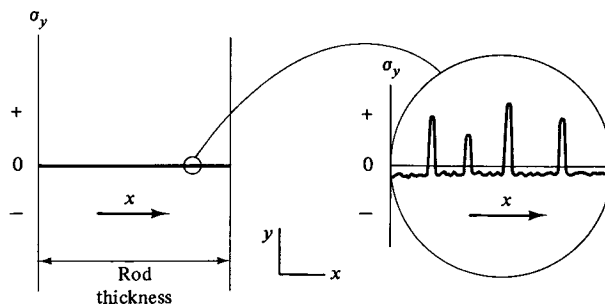
Fig. 9.33 Distribution of longitudinal residual stress across the diameter of a rod after plastic elongation in the y direction.
