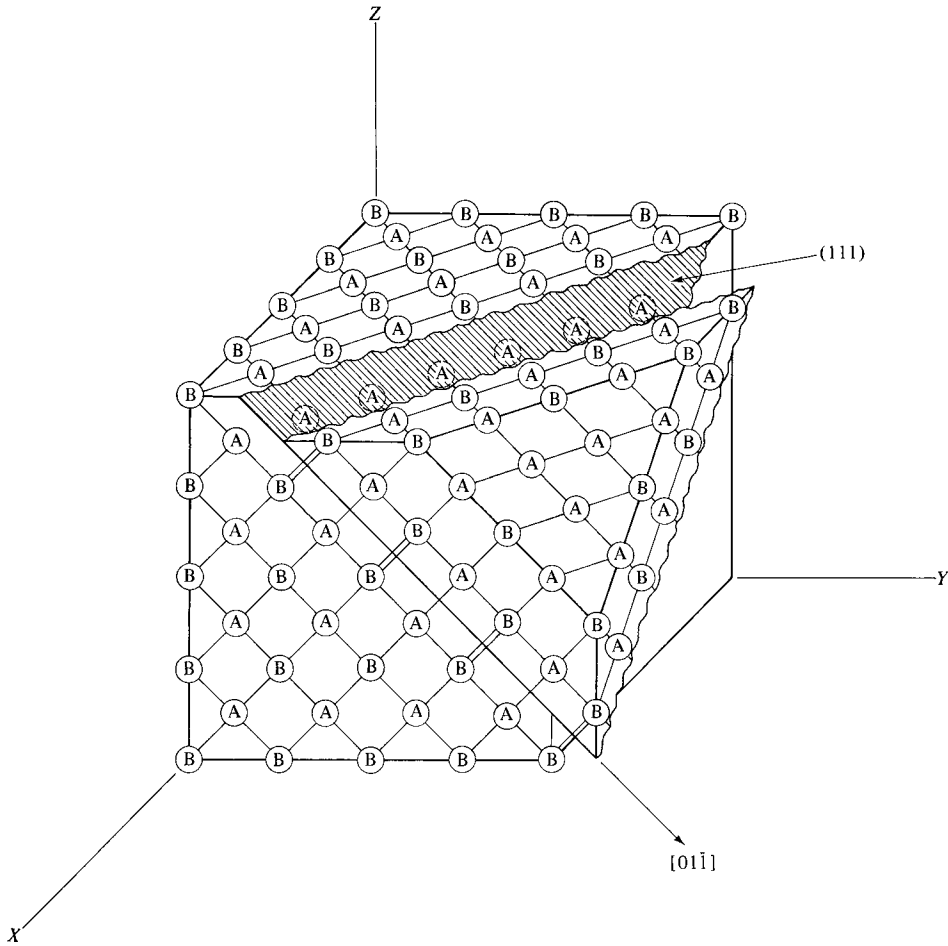
Fig. 10.13 Formation of AA and BB pairs by slip in an A_3B superlattice. [S. Chikazumi, Physics of Magnetism , Oxford University Press (1997).]
