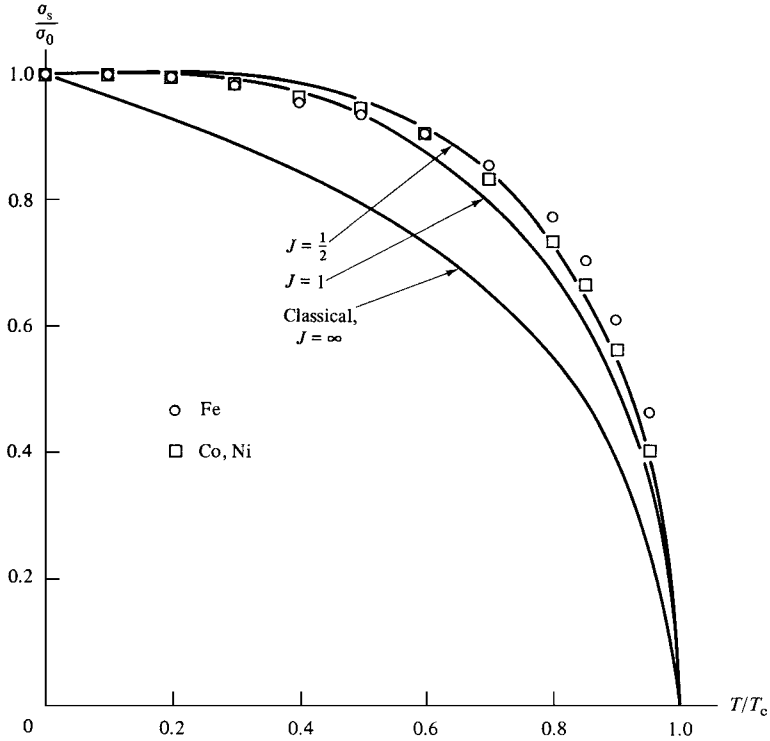
Fig. 4.7 Relative saturation magnetization of iron, cobalt, and nickel as a function of relative temperature. Calculated curves are shown for three values of J .
