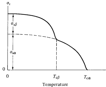
Fig. 4.24 Variation of \sigma_s with temperature in an alloy of two ferromagnetic phases.
