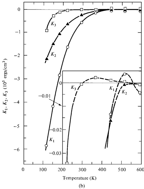
Fig. 7.24 Temperature dependence of anisotropy constants. (a) Iron [K. Honda, H. Masumoto, and S. Kaya, Sci. Rep. Tohoku Univ. , 17 (1928) p. 111]. (b) Nickel [G. Aubert, J. Appl. Phys. , 39 (1968) p. 504].
