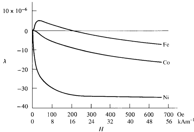
Fig. 8.13 Magnetostriction of polycrystalline iron, cobalt, and nickel. [E. W. Lee, Rep. Progr. Phys. , 18 (1955) p. 184.]
