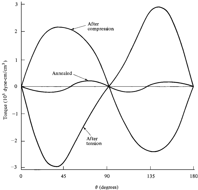
Fig. 10.14 Torque curves for annealed nickel and for nickel after plastic tension and compression of 2.5%. [After R. F. Krause and B. D. Cullity, J. Appl. Phys. , 39 (1968) p. 5532.]
