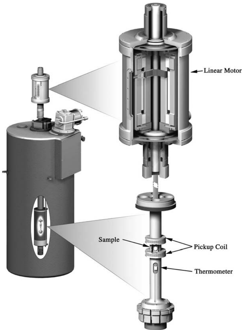
Fig. 2.38 VSM working in a superconducting solenoid. The oscillating sample motion is provided by a linear motor. Courtesy of Quantum Design, Inc.
