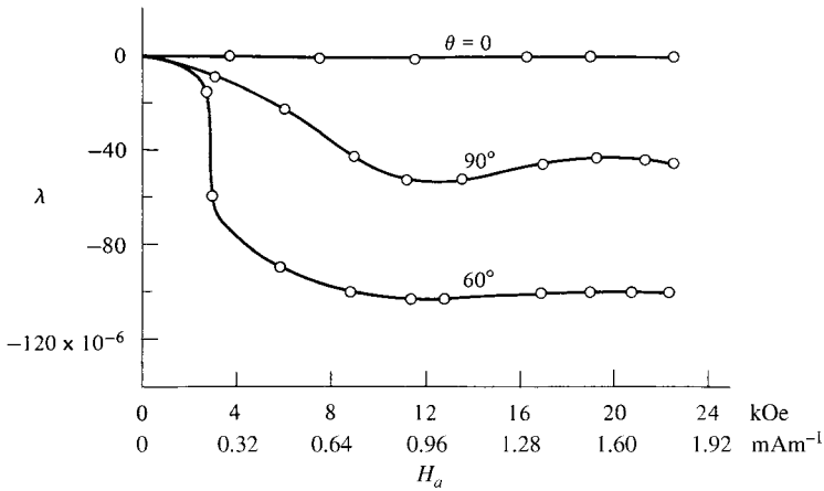
Fig. 8.9 Magnetostriction of a cobalt single crystal as a function of field. The strain \lambda is measured parallel to the field H , and \theta is the angle between them and the hexagonal axis. [R. M. Bozorth, Ferromagnetism , reprinted by IEEE Press (1993).]
