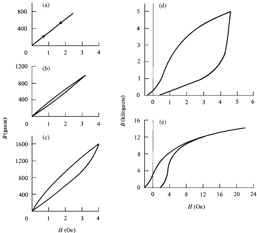
Fig. 10.8 Hysteresis loops of Perminvar annealed at 425°C. [R. M. Bozorth, Ferromagnetism , reprinted by IEEE Press (1993).]
