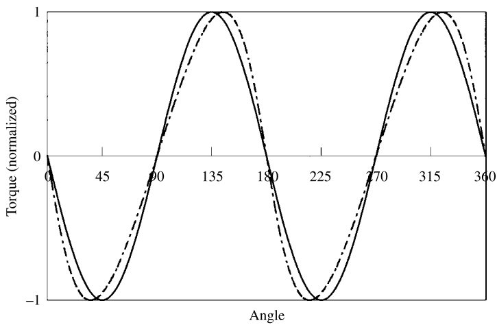
Fig. 7.12 Variation of torque with angle \psi between easy axis c and field H for a uniaxial crystal. The dashed curve is for H = 2K_1/M_s ; solid curve for H \gg 2K_1/M_s .
