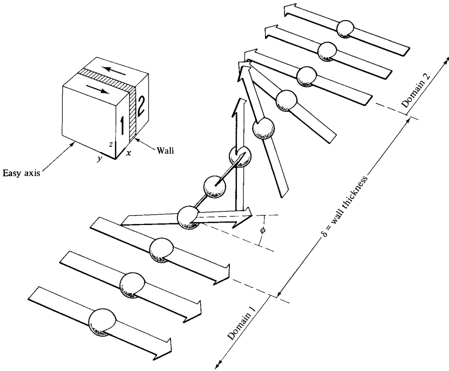
Fig. 9.2 Structure of a 180^\circ domain wall.
