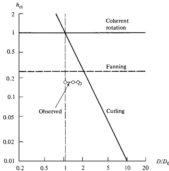
Fig. 11.9 Calculated reduced coercivities for coherent and curling reversals in an infinite cylinder, and for fanning reversal in an infinite chain of spheres, as a function of the reduced diameter D/D_0 . Crystal anisotropy is neglected. The observed values are for elongated iron particles. [F. E. Luborsky, J. Appl. Phys. , 32 (1961) p. 171S.]
