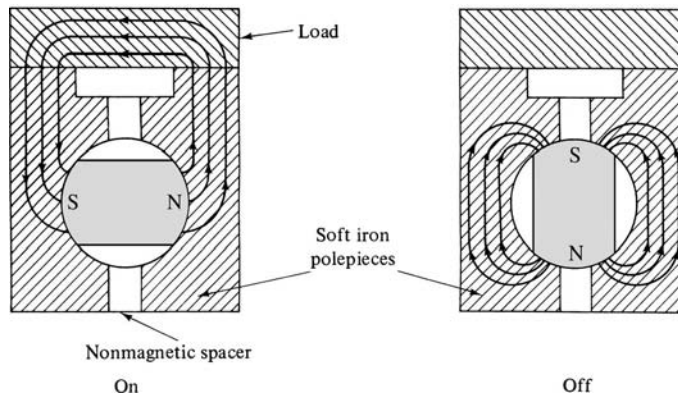
Fig. 14.20 Permanent magnet chuck.
