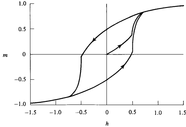
Fig. 9.37 Hysteresis loop of an assembly of noninteracting, randomly oriented, uniaxial single domain particles.
