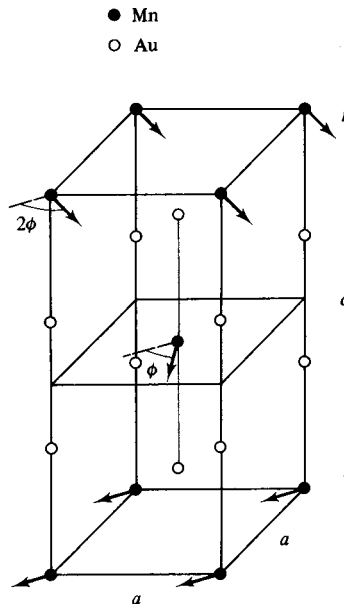
Fig. 5.17 Structure of \text{MnAu}_2 .
