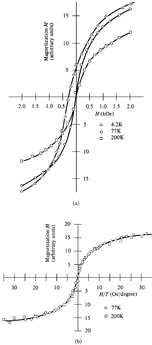
Fig. 11.18 Magnetization curves of iron particles 44 A in diameter. [I. S. Jacobs and C. P. Bean, Magnetism , Volume 3, G. T. Rado and H. Suhl, eds., Academic Press (1966).]
