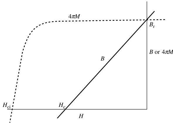
Fig. 14.7 Demagnetizing behavior of a high H_{ci} permanent magnet. The magnetization is unchanged by negative fields less than H_c , so H_c = B_r (in cgs units).
