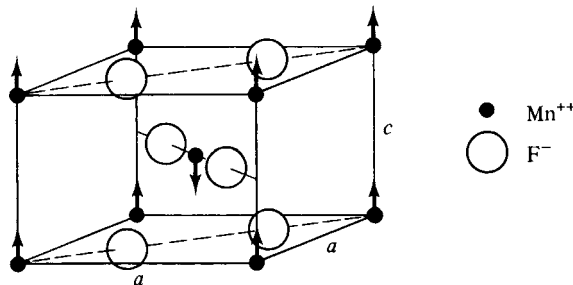
Fig. 5.12 Structure of \text{MnF}_2 .
