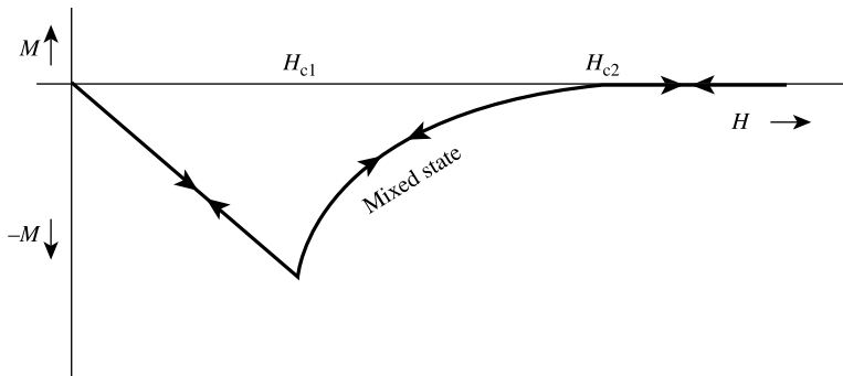
Fig. 16.4 Magnetic behavior of an ideal type II superconductor ( N = 0 ).
