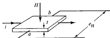
Fig. 2.15 Sketch of a Hall plate, showing the relationship between field, current, and emf.
