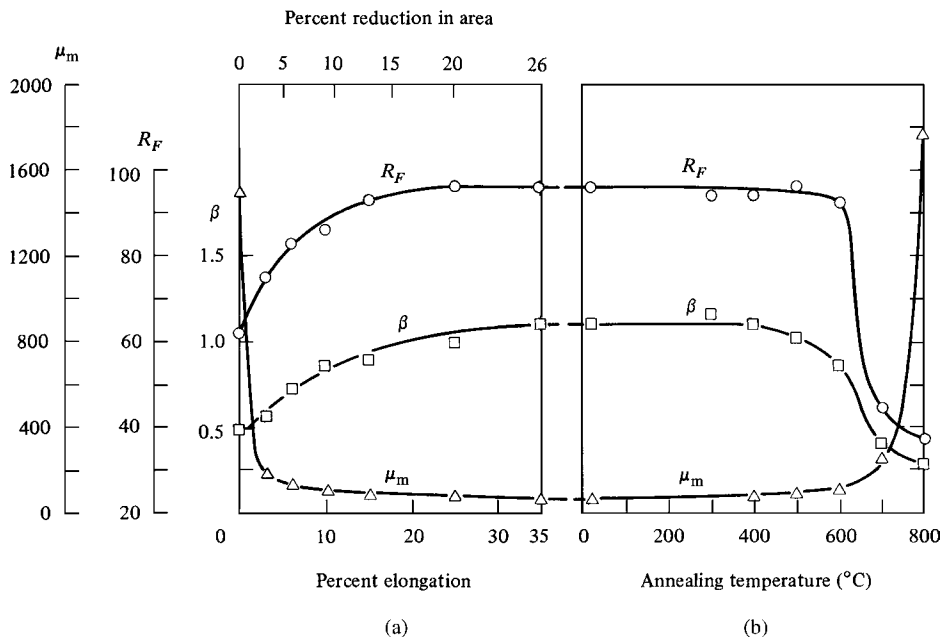
Fig. 9.46 Changes in physical properties of nickel during tensile deformation and subsequent annealing. R_F = hardness on Rockwell F scale; \beta = width (degrees) of the (420) X-ray line, using \text{Cu K}\alpha_1 radiation; \mu_m = maximum permeability. [H. Chou and B. D. Cullity, unpublished.]
