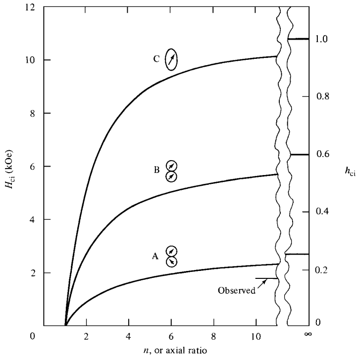
Fig. 11.7 Calculated coercivities for aligned n -sphere chains (A and B) and prolate spheroids of axial ratio n (C). The observed values are for elongated iron particles. [F. E. Luborsky, J. Appl. Phys. , 32 (1961) p. 171S.]
