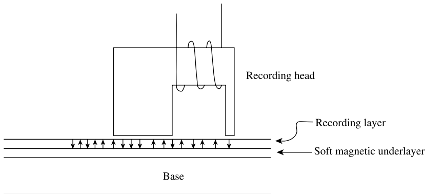
Fig. 15.7 Perpendicular recording geometry.
