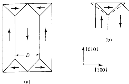
Fig. 9.18 Closure domains in a cubic crystal with \langle 100 \rangle easy axes.
