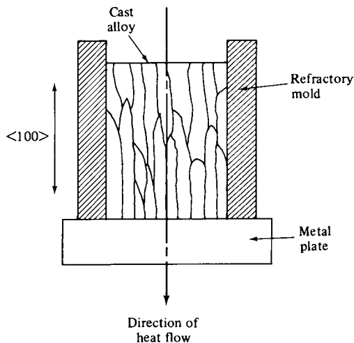
Fig. 14.10 Directional solidification of alnico to produce columnar grains oriented in the \langle 100 \rangle direction.
