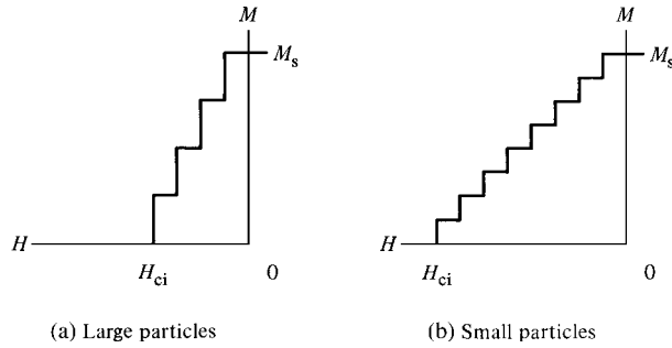
Fig. 11.17 Demagnetization curves of assemblies of particles.
