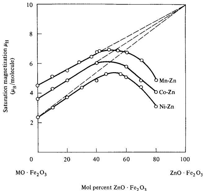
Fig. 6.4 Effect on the saturation moment (at 0K) of adding Zn ferrite to Mn, Co, and Ni ferrite.
