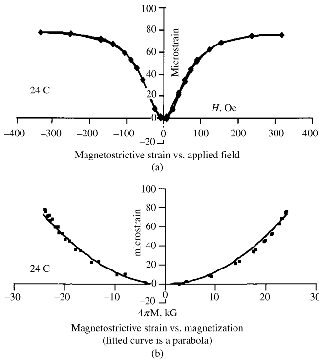
Fig. 8.14 Magnetostriction vs field and vs magnetization for polycrystalline FeCo + 2% V. [B. E. Lorenz and C. D. Graham, IEEE Trans. Mag. , 42 (2006) p. 3886.]
