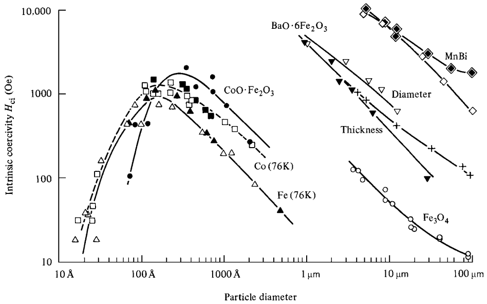
Fig. 11.1 Variation of coercivity with particle size, for particles whose coercivity depends on crystal anisotropy. [F. E. Luborsky, J. Appl. Phys. , 32 (1961) p. 171S.]
