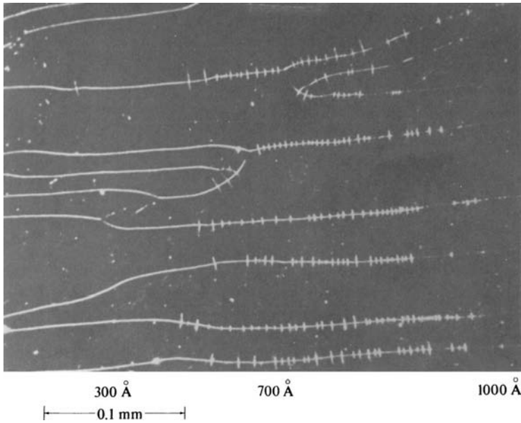
Fig. 11.35 Domain walls in a tapered film of 80 permalloy. Easy axis horizontal. Dark-field Bitter pattern. [S. Methfessel et al., J. Appl. Phys. , 31 (1960) p. 302S.]
