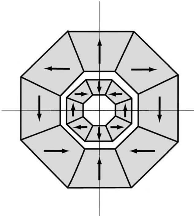
Fig. 2.14 Pair of concentric Halbach arrays. Each array can be rotated independently about the central axis perpendicular to the page.
