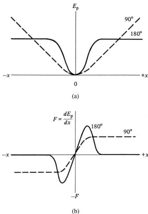
Fig. 10.7 (a) Potential energy E_p as a function of the displacement x of 90^\circ and 180^\circ walls from a stabilized position. (b) Force F required to move the wall (schematic).
