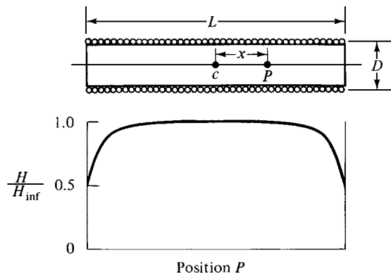
Fig. 2.1 Single-layer solenoid and its field distribution. The axial field at point P is expressed as the fraction of the field at the center of an infinitely long solenoid.
