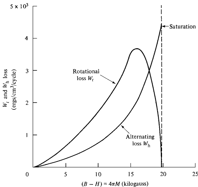
Fig. 13.10 Dependence on 4\pi M of the rotational hysteresis loss W_r and the alternating hysteresis loss W_h in the rolling direction for grain-oriented 3.13% silicon steel. [F. Brailsford, J. Inst. Elect. Engrs , 84 (1939) p. 399.]
