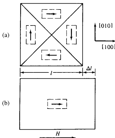
Fig. 8.2 Magnetostriction of an iron crystal in the [100] direction.
