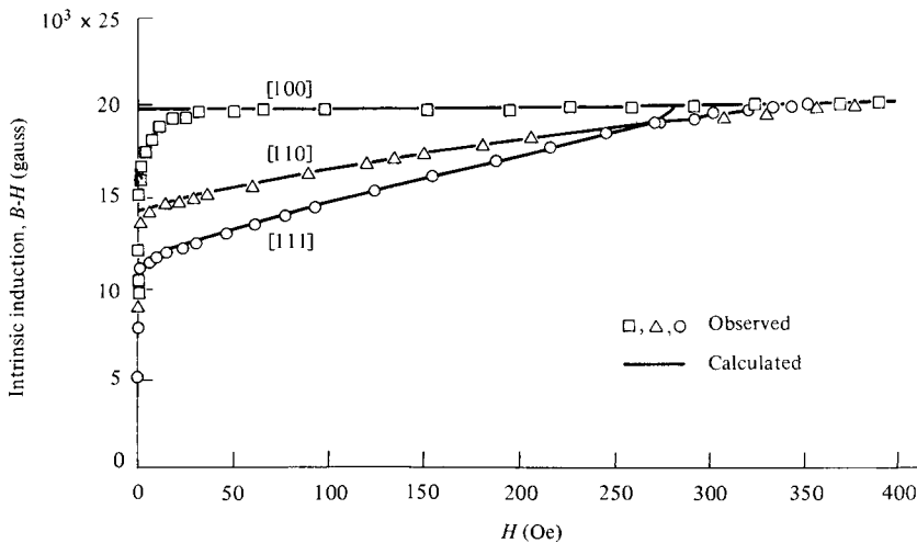
Fig. 7.22 Calculated and measured magnetization curves for Fe-Si crystals. [R. M. Bozorth, Ferromagnetism , reprinted by IEEE Press (1993).]
