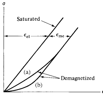
Fig. 8.26 Elastic and magnetoelastic contributions to the stress–strain curve.
