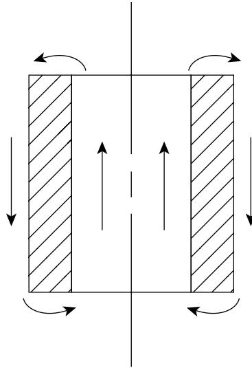
Fig. 16.7 Field distribution around a superconducting solenoid.
