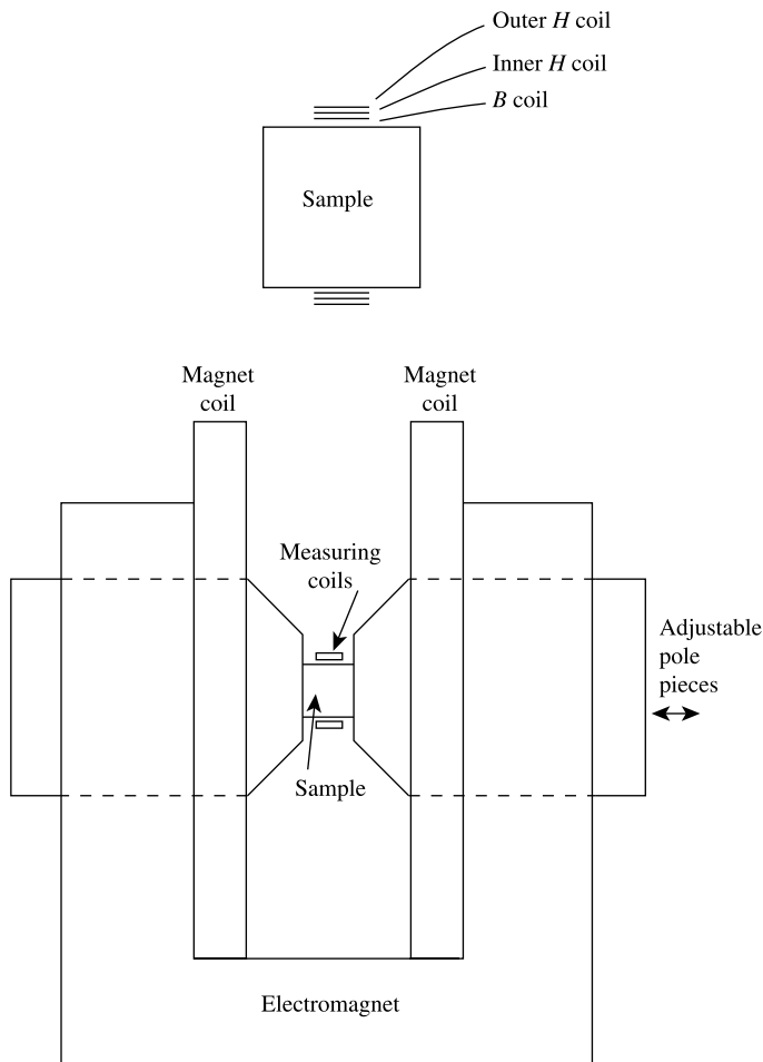
Fig. 2.44 Measurement of permanent magnet sample (schematic).
