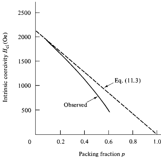
Fig. 11.3 Variation of H_{ci} with p for elongated Fe–Co particles. [After F. E. Luborsky J. Appl. Phys. , 32 (1961) p. 171S.]
