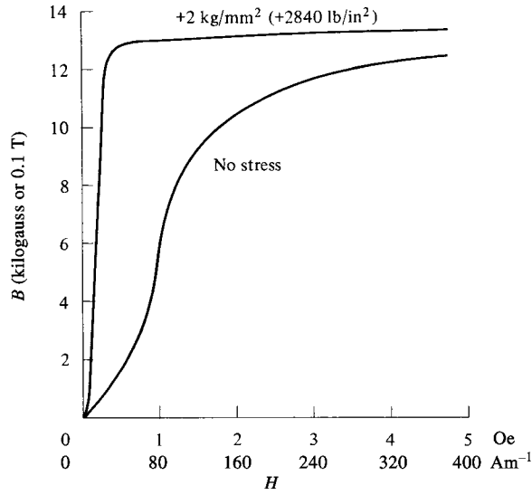
Fig. 8.17 Effect of applied tensile stress on the magnetization curve of 68 permalloy. [R. M. Bozorth, Ferromagnetism , reprinted by IEEE Press (1993).]
