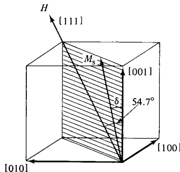
Fig. 7.20 Magnetization of an iron crystal in a [111] direction.
