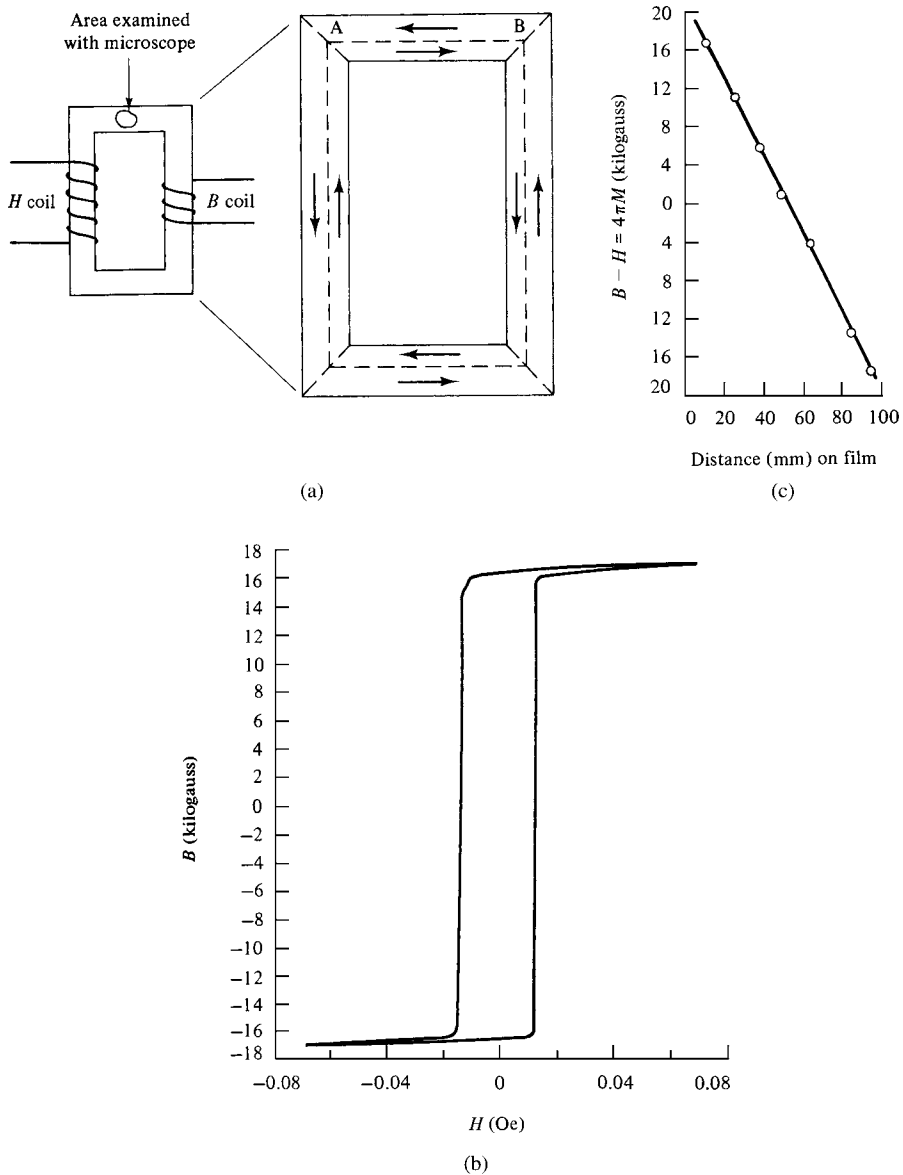
Fig. 9.24 The picture-frame experiment. [H. J. Williams and W. Shockley, Phys. Rev. , 75 (1949) p. 178.]
