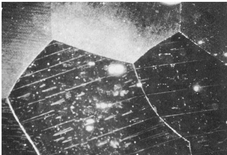
Fig. 9.22 Domains in a polycrystalline sample of Fe + 3% Si.
