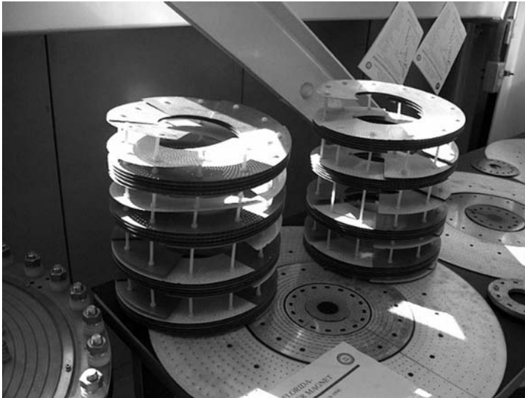
Fig. 2.6 Photograph of partially-assembled Bitter magnets. Figures 2.6 and 2.7 are by Walter Thorne, National High Magnetic Field Laboratory.
