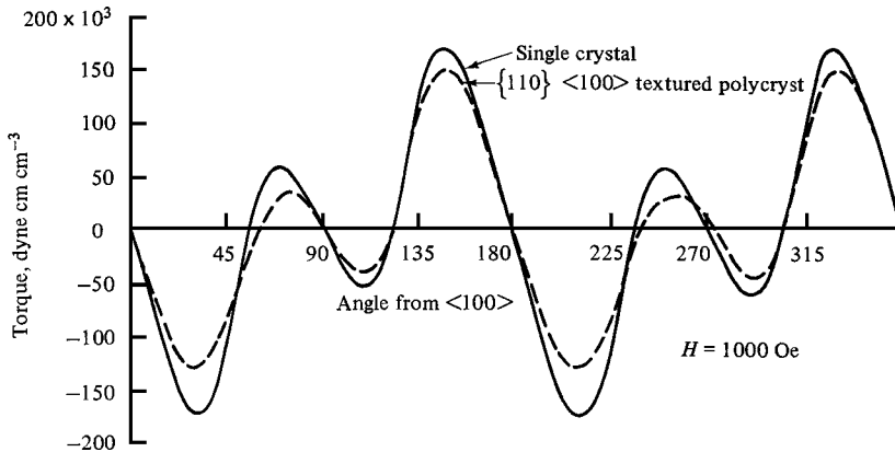
Fig. 13.15 Torque curves of a single crystal in the {110} plane and of a disk cut from a sheet of grain-oriented silicon steel having a strong cube-on-edge, {110} <100> texture. [C. D. Graham, Magnetism and Metallurgy , Volume 2, Academic Press (1969).]
