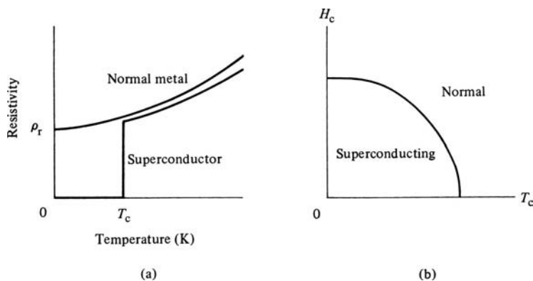
Fig. 2.8 (a) Variation of electrical resistivity with temperature for a normal metal and a superconductor. (b) Dependence of critical temperature on magnetic field.
