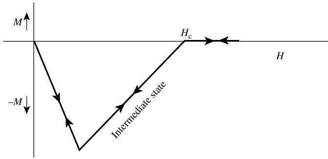
Fig. 16.2 Magnetic behavior of an ideal type I superconductor with nonzero demagnetizing factor N .
