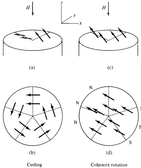
Fig. 11.8 (a) and (c) are curling and coherent-rotation modes. (b) and (d) are cross sections normal to the z axis after a 90^\circ rotation from the +z direction.
