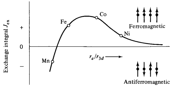
Fig. 4.13 Bethe–Slater curve (schematic).
