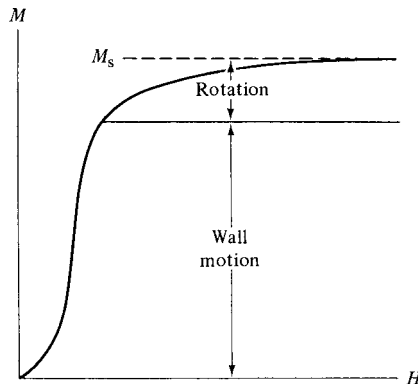
Fig. 9.25 Magnetization processes.
