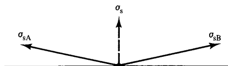
Fig. 5.18 Canted spins.
