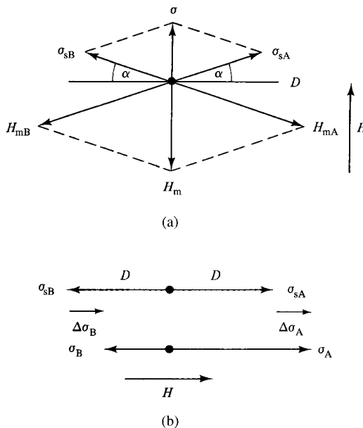
Fig. 5.5 Magnetization changes in an antiferromagnet when the field H is applied (a) at right angles and (b) parallel to the spin axis D .
