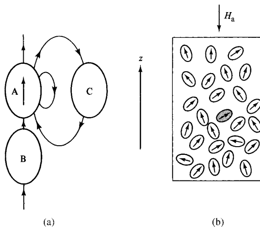
Fig. 11.4 Particle interactions.
