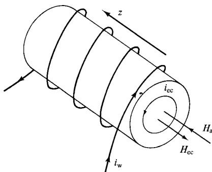
Fig. 12.1 Eddy currents in a rod.
