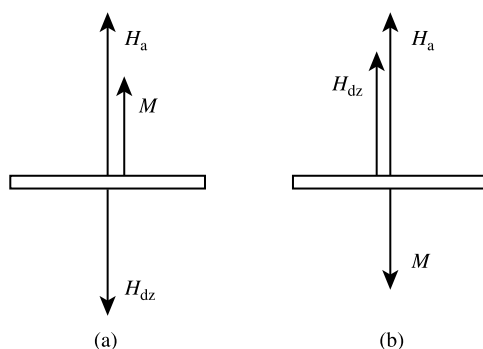
Fig. 16.8 Demagnetizing fields acting on a thin film sample with the applied field H_a perpendicular to the sample plane. H_{dz} is the demagnetizing field perpendicular to the sample plane. (a) Ferromagnet ( \chi \gg 1 ). The perpendicular demagnetizing field H_{dz} is large because of the large perpendicular demagnetizing factor, and this field acts to decrease the magnetization of the sample. (b) Superconductor ( \chi = -1 ). The large perpendicular demagnetizing field in this case acts to increase the perpendicular component of magnetization.
