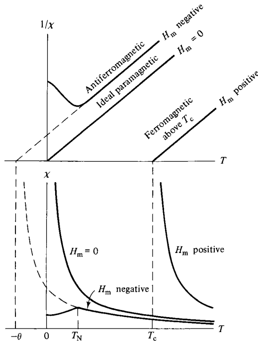
Fig. 5.3 Dependence of the susceptibility \chi on the molecular field H_m for a fixed value of the Curie constant C .
