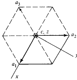
Fig. 8.8 Hexagonal and orthogonal axes in a hexagonal crystal.
