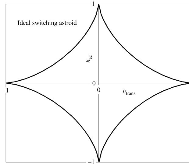
Fig. 12.9 Ideal switching astroid.
