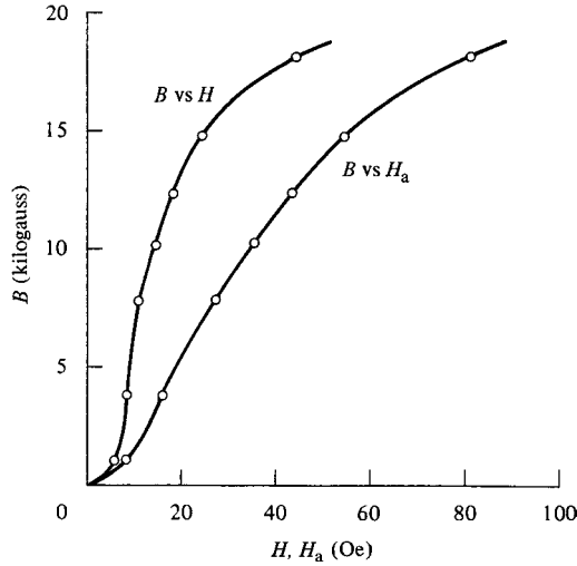
Fig. 2.34 Measured and corrected magnetization curves of cold-worked iron, from the data of Table 2.2.
