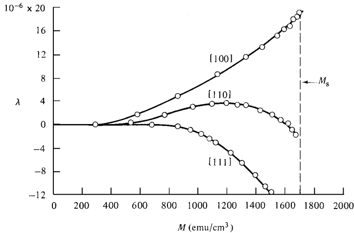
Fig. 8.5 Magnetostriction as a function of magnetization in single crystal iron rods. Each rod had a different crystallographic axis. [W. L. Webster, Proc. R. Soc. , A109 (1925) p. 570.]
