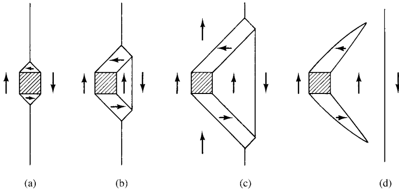
Fig. 9.29 Passage of a domain wall through an inclusion.
