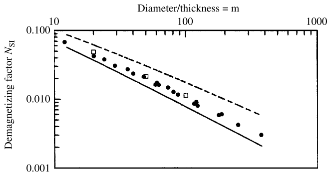
Fig. 2.31 Magnetometric demagnetizing factors for disk samples. Data points measured on 80 permalloy disk samples using a vibrating-sample magnetometer [C. D. Graham and B. E. Lorenz, IEEE Trans. Mag. , 43 (2007) p. 2743]. Dotted and solid lines are copied from Fig. 2.30, for \chi = \infty and \chi = 0 .
