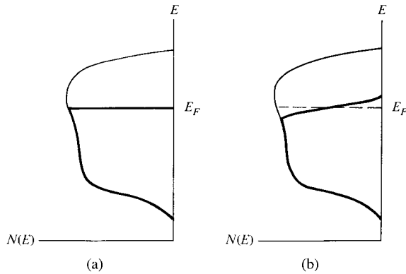
Fig. 4.19 Electron distributions at (a) 0K and (b) at a high temperature. E_F is the Fermi level.
