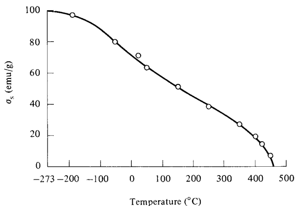
Fig. 6.13 Temperature variation of saturation magnetization of barium ferrite.
