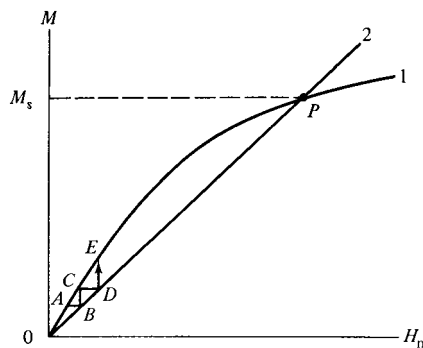
Fig. 4.3 Spontaneous magnetization by the molecular field.
