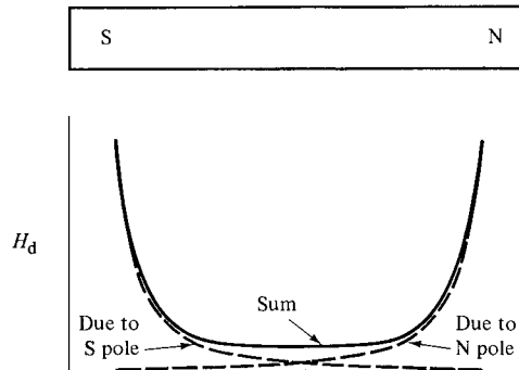
Fig. 2.22 Variation of the demagnetizing field along the length of a bar magnet.
