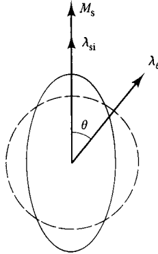
Fig. 8.7 Isotropic magnetostriction.
