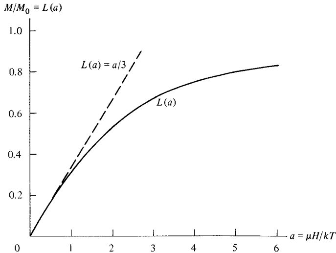
Fig. 3.3 Langevin function.
