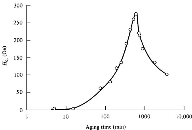
Fig. 11.24 Effect of aging at 700°C on the coercivity H_{ci} of a Cu–Co alloy. [J. J. Becker, Trans. AIME , 209 (1957) p. 59.]
