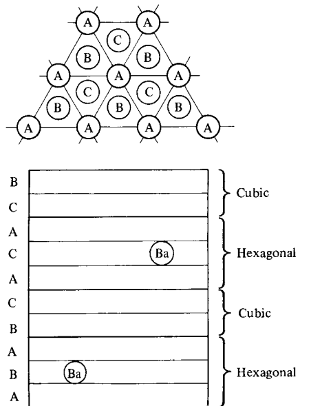
Fig. 6.12 The barium ferrite structure.
