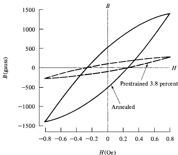
Fig. 9.45 Hysteresis loops for polycrystalline iron, calculated from measured Rayleigh constants.
