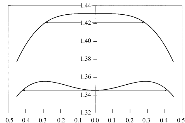
Fig. 2.4 Field distribution in a “pure” Helmholtz coil (upper curve) compared with field distribution in a Helmholtz coil pair whose coil spacing has been increased by 10%. The dimension lines show the distance over which the field is uniform within 0.7% of the maximum field.
