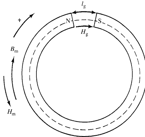
Fig. 14.2 Open magnetic circuit.
