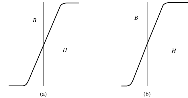
Fig. 2.17 Principle of fluxgate magnetometer (schematic).
