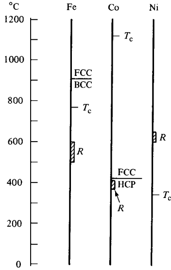
Fig. 4.6 Curie points ( T_c ), recrystallization temperatures [ R ], and phase changes in Fe, Co, and Ni. BCC = body-centered cubic; FCC = face-centered cubic; HCP = hexagonal close packed. Ni is FCC at all temperatures.
