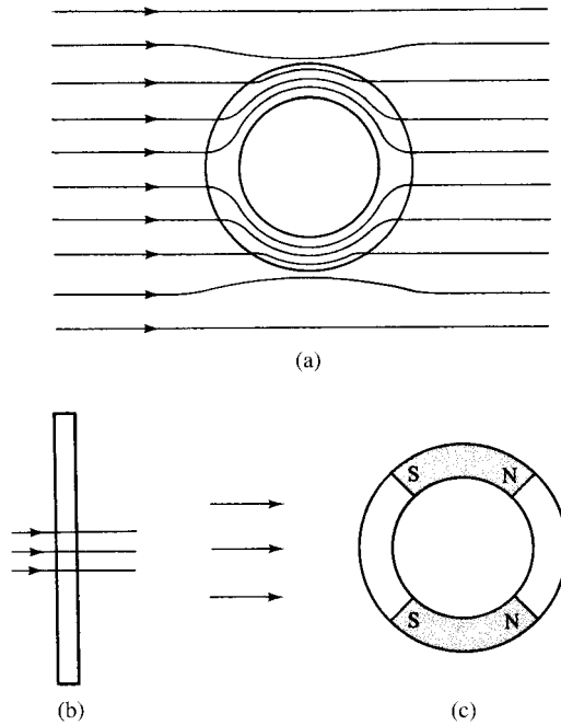
Fig. 2.25 Magnetic shielding.
