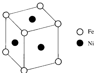
Fig. 10.6 The ordered form of FeNi 3 .
