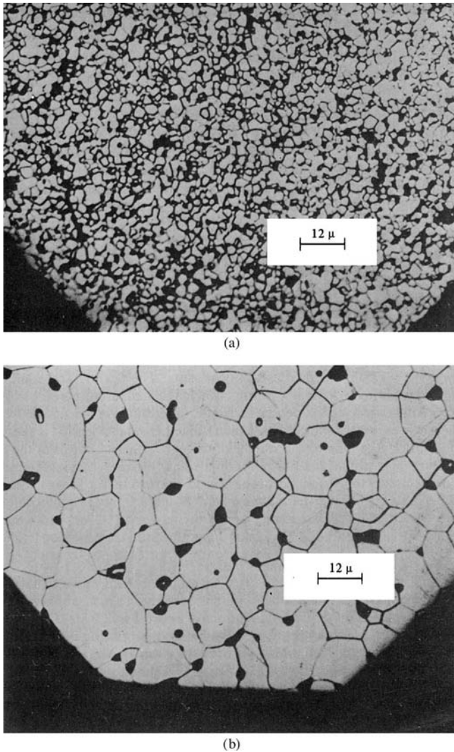
Fig. 13.25 Microstructure of a Mn–Zn ferrite. (a) After sintering 5 min at 1375°C (10% porosity). (b) After sintering 1 min at 1435°C (5% porosity). [Figures 13.25, 13.26, and 13.27 are from J. Smit and H. P. J. Wijn, Ferrites , Wiley (1959).]
