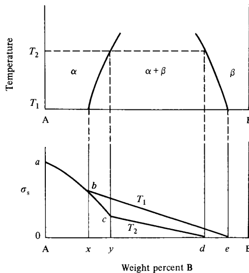
Fig. 4.23 Variation of saturation magnetization \sigma_s with composition in alloys equilibrated at temperatures T_1 and T_2 .
