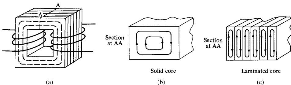
Fig. 13.1 Eddy currents in a transformer core.
