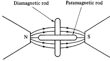
Fig. 2.46 Orientations of para- and diamagnetic rods in the field of an electromagnet.
