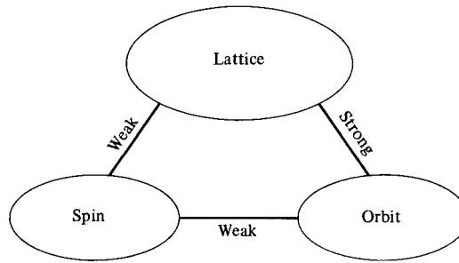
Fig. 7.8 Spin–lattice–orbit interactions.
