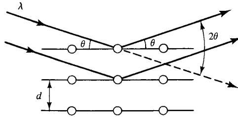
Fig. 5.10 Diffraction geometry.
