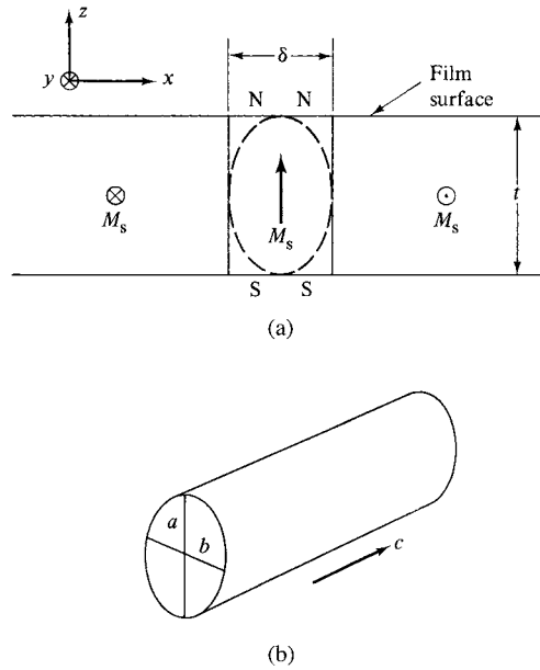
Fig. 11.30 (a) Cross section of 180° Bloch wall in thin film. (b) Elliptic cylinder.
