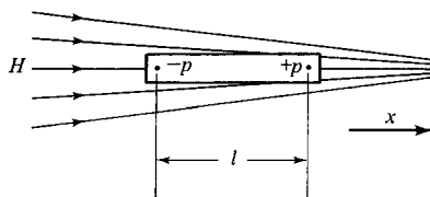
Fig. 2.45 Magnetized body in a nonuniform field.
