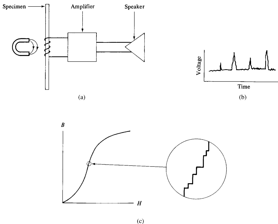
Fig. 9.23 Barkhausen effect.
