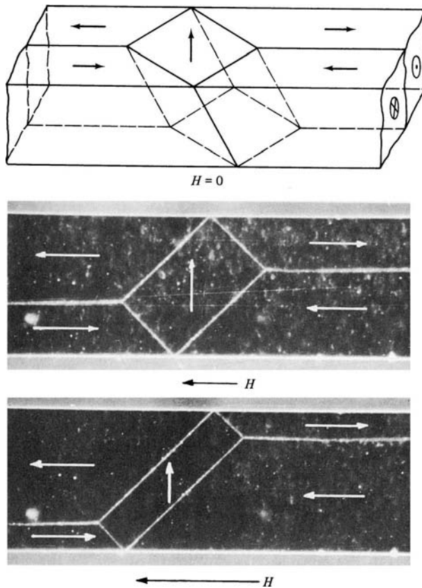
Fig. 9.20 Reversible wall motion in an iron whisker. Bitter patterns under dark-field illumination.
