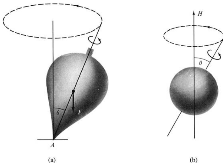
Fig. 3.6 Precession of (a) a spinning top in a gravitational field, and (b) a magnetic atom in a magnetic field.
