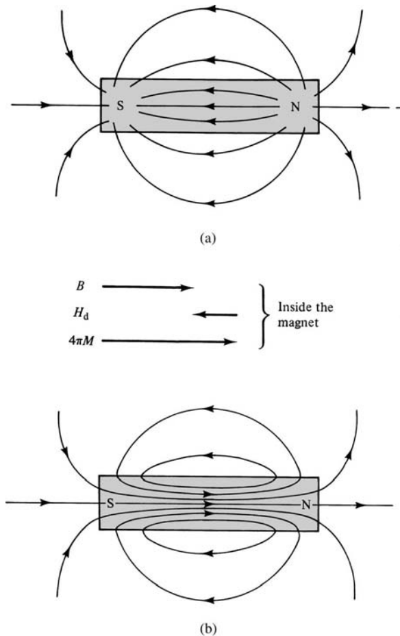
Fig. 2.21 Fields of a bar magnet in zero applied field. (a) H field, and (b) B field. The vectors in the center indicate the values and directions of B , H_d , and 4\pi M (cgs units) at the center of the magnet.
