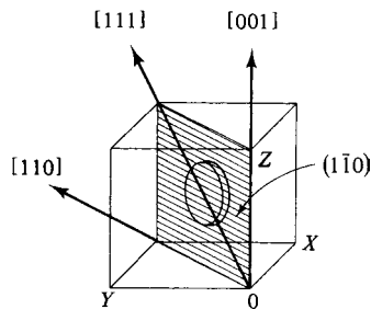
Fig. 7.1 The three principal crystallographic directions in the (1\bar{1}0) plane of a cubic material.
