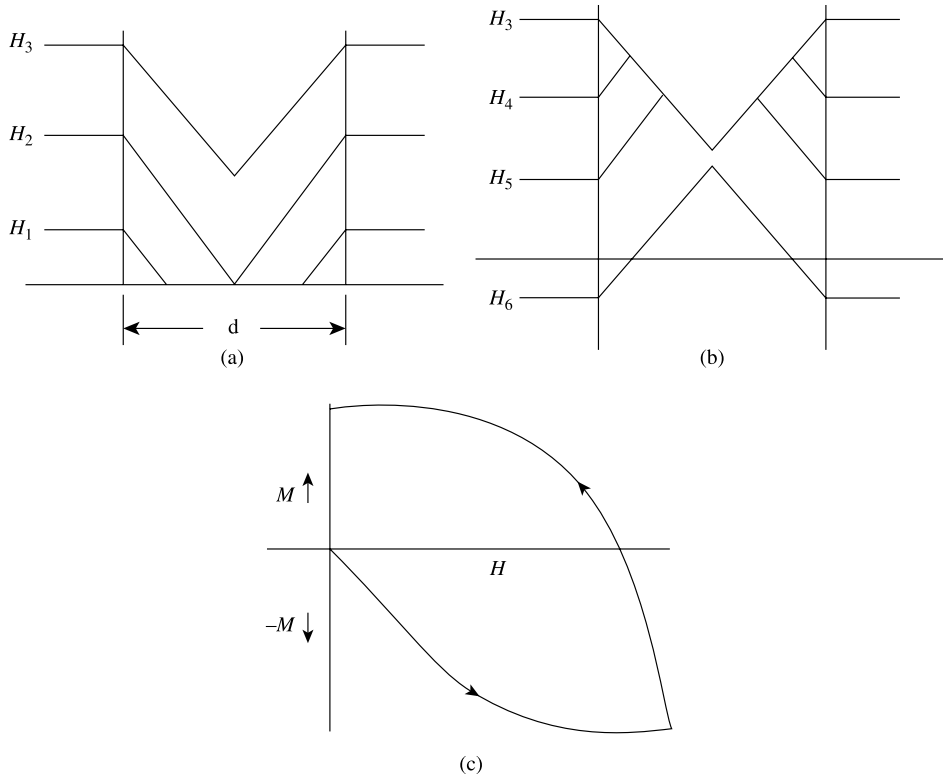
Fig. 16.5 Field penetration in a type II hard (flux-pinned) superconductor slab of thickness d , according to the Bean model. (a) Applied field increasing in steps H_1 , H_2 , H_3 . (b) Field decreasing in steps H_3 , H_4 , H_5 , H_6 . (c) Resulting magnetization behavior.
