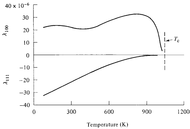
Fig. 8.10 Temperature dependence of magnetostriction constants of iron. [T. Okamoto and E. Tatsumoto, J. Phys. Soc. Japan , 14 (1959) p. 1588.]
