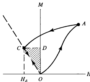
Fig. 7.29 Magnetostatic energy of a magnetized body in zero applied field.
