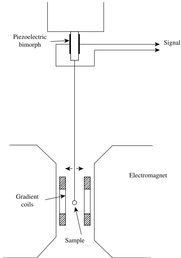
Fig. 2.39 Alternating-gradient magnetometer or AGM (schematic).
