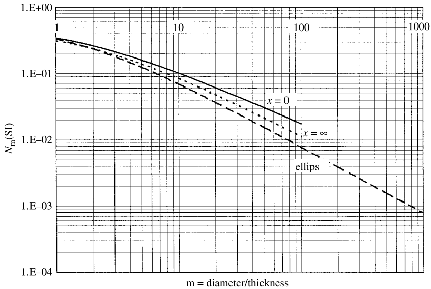
Fig. 2.30 Calculated SI magnetometric demagnetizing factors for disk samples magnetized along a diameter. Dashed line is for an oblate (planetary) ellipsoid. Dotted line is N_m for \chi = \infty ; solid line is for \chi = 0 .
