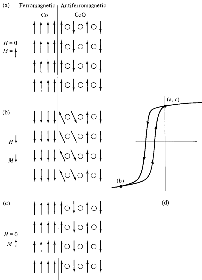
Fig. 11.27 Mechanism of the shifted loop in Co–CoO. Arrows represent spins on cobalt atoms or ions, and open circles are oxygen ions. Points (a)–(c) on the loop correspond to the three states at the left.
