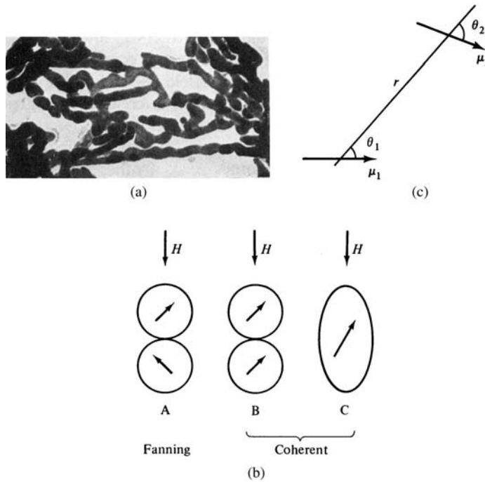
Fig. 11.5 (a) Electron micrograph of electrodeposited iron particles [F. E. Luborsky, J. Appl. Phys. , 32 (1961) p. 171S]. (b) Models of particle shape and reversal modes. (c) Dipole–dipole interactions.
