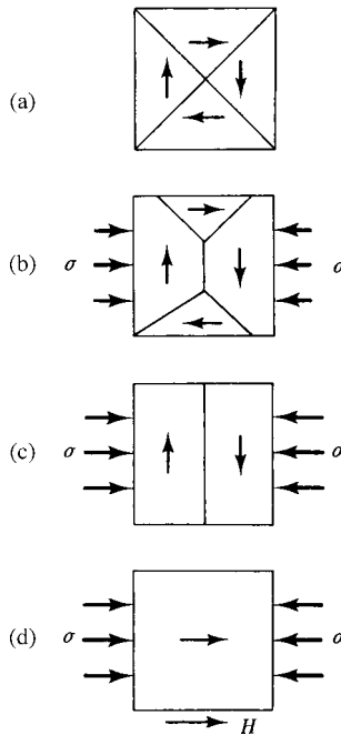
Fig. 8.22 Magnetization of a material with positive magnetostriction under compressive stress (schematic).
