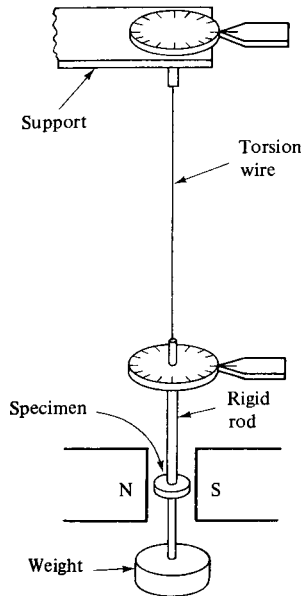
Fig. 7.16 Basic mechanical torque magnetometer (schematic).
