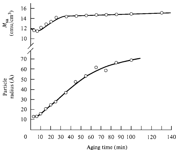
Fig. 11.23 Effect of aging at 650°C on the saturation magnetization M_{sa} of a Cu–Co alloy and on the effective radius R of the precipitate particles. [J. J. Becker, Trans. AIME , 209 (1957) p. 59.]
