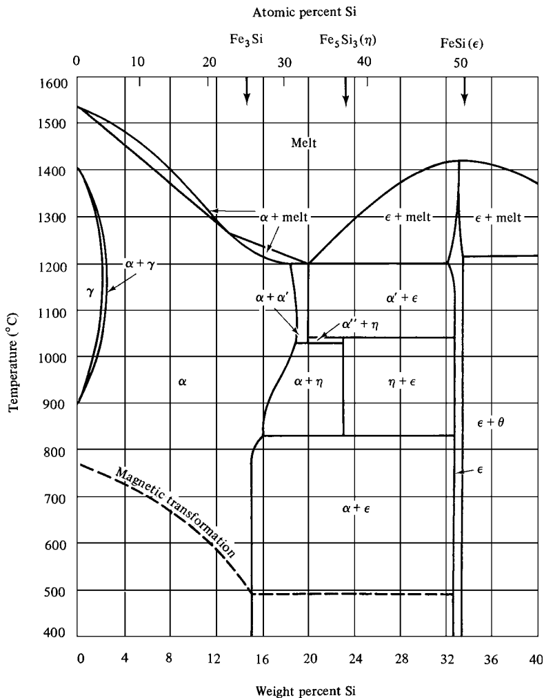
Fig. 13.11 Portion of iron–silicon equilibrium diagram.
