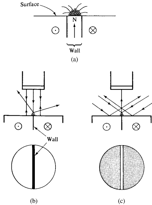
Fig. 9.8 Bitter method or powder method for observation of domain walls.
