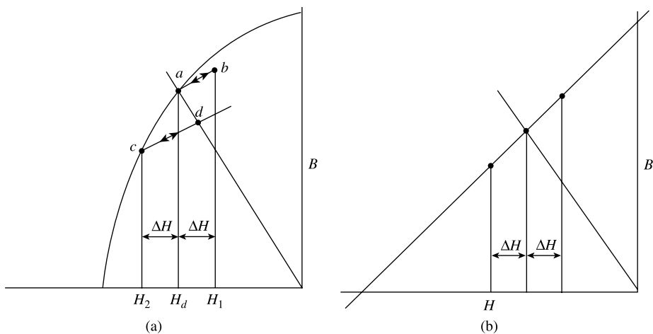
Fig. 14.15 Stabilization of a permanent magnet.
