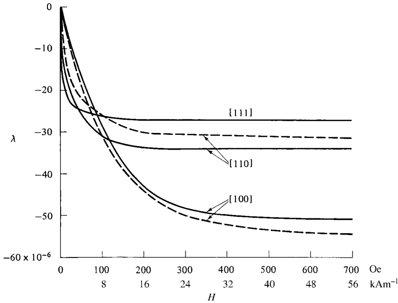
Fig. 8.6 Magnetostriction as a function of field and crystal direction for nickel single crystal. Samples were planetary (oblate) spheroids. Solid lines, {011} disk; dashed lines, [001] disk. [Y. Masiyama, Sci. Rep. Tohoku Univ. , 17 (1928) p. 947.]
