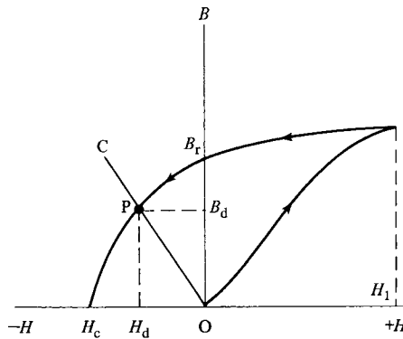
Fig. 14.1 Initial magnetization and demagnetization curve of a permanent magnet. B_r is the residual induction; point P is the operating point.
