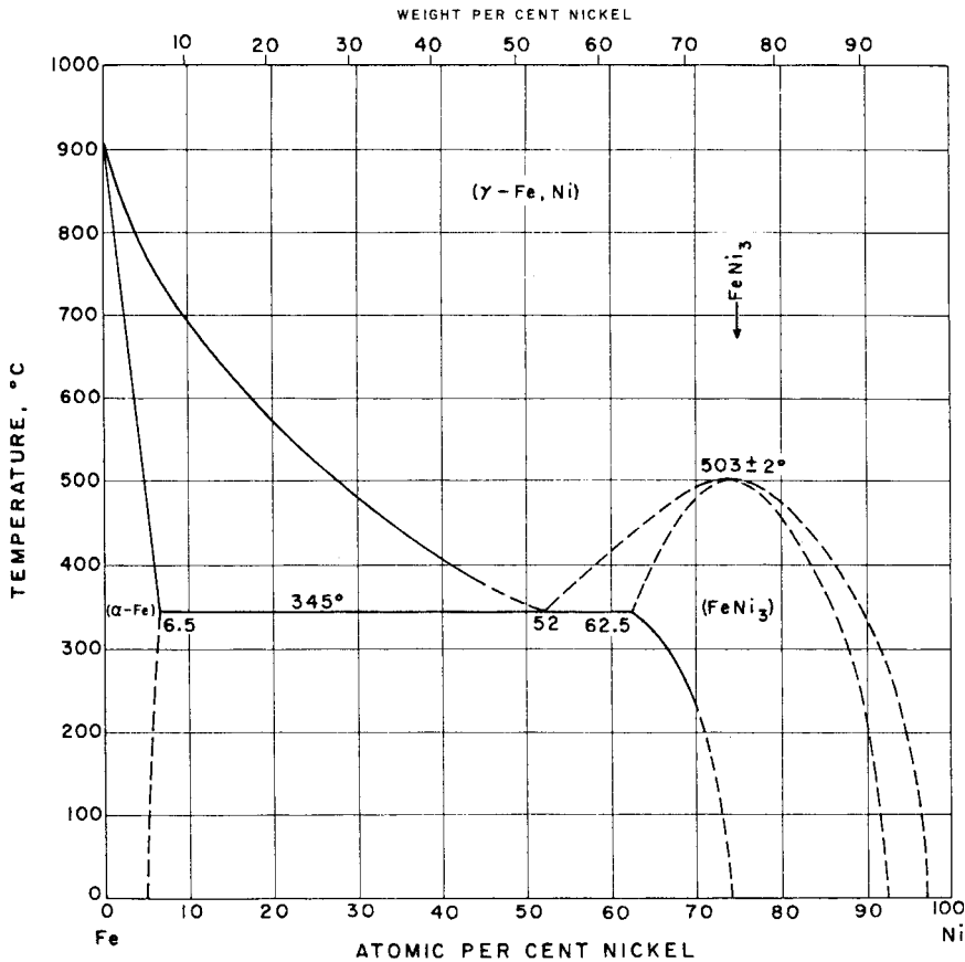
Fig. 10.1 Equilibrium phase diagram of Fe–Ni alloys. [E. J. Swartzendruber, V. P. Itkin, and C. B. Alcock, ASM Handbook , Volume 3 (1992).]
