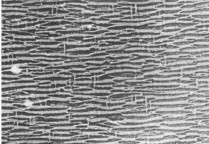
Fig. 14.9 Electron micrograph (oxide replica) from a single crystal of field-annealed alnico. The field during annealing was directed horizontally; 50,000 \times [K. J. De Vos, Magnetism and Metallurgy , Volume 2, Academic Press (1969)].
