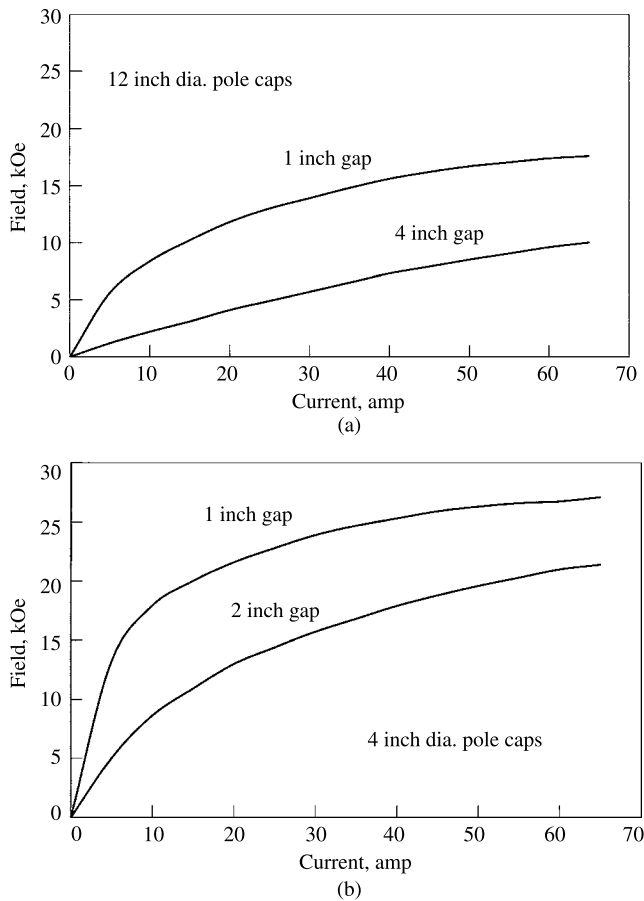
Fig. 2.11 Magnetic field (kOe) vs current in a 12-inch electromagnet: (a) 4-inch and 1-inch gaps; (b) with 4-inch tapered pole caps, 2-inch and 1-inch gaps.
