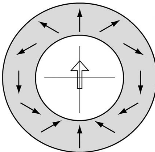
Fig. 2.12 Halbach cylinder. Solid arrows show direction of local magnetization. The open arrow is the resulting field.
