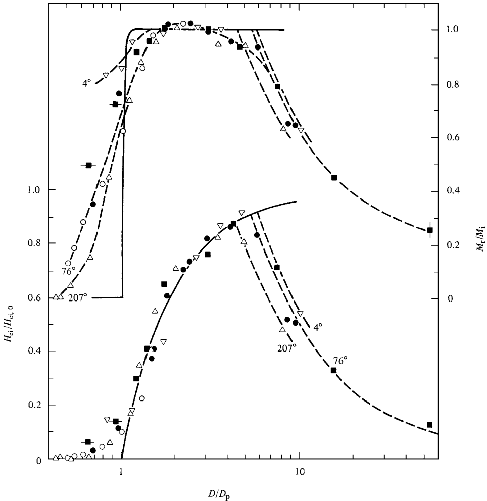
Fig. 11.20 Particle size dependence of the coercivity (lower curve) and retentivity (upper curve) of a Co-Fe alloy. Solid lines are calculated. [E. F. Kneller and F. E. Luborsky, J. Appl. Phys. , 34 (1963) p. 656.]
