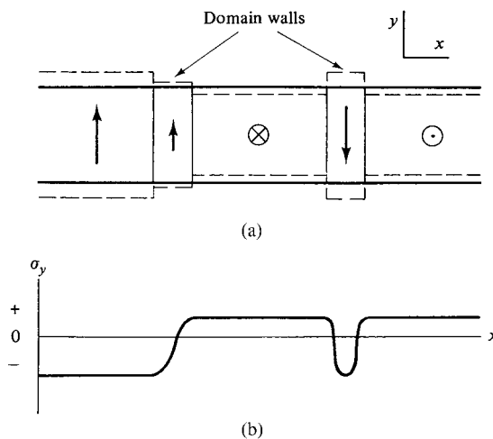
Fig. 9.31 Microstresses due to magnetostriction.
