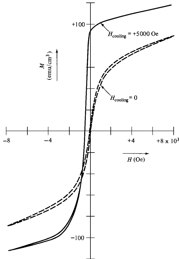
Fig. 11.26 Hysteresis loops measured at 4.2K of an alloy of Ni + 26.5 atomic percent Mn after cooling with and without a field of 5 kOe in the positive direction. [J. S. Kouvel, C. D. Graham, and I. S. Jacobs, J. Phys. Rad. , 20 (1959) p. 198.]
