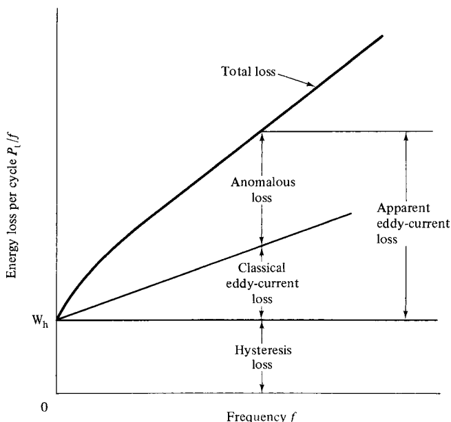
Fig. 13.7 Conventional separation of losses in transformer cores.
