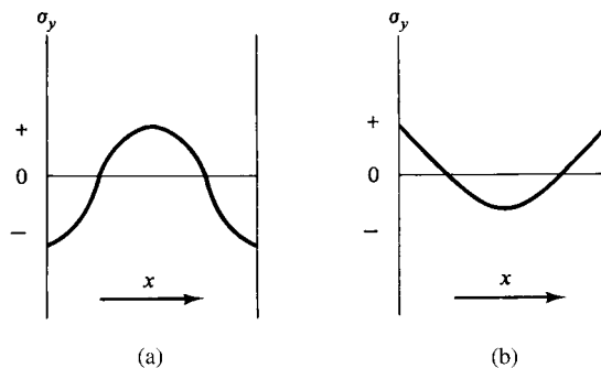
Fig. 9.32 Possible distributions of longitudinal residual stresses across the diameter of a cold-drawn metal rod.
