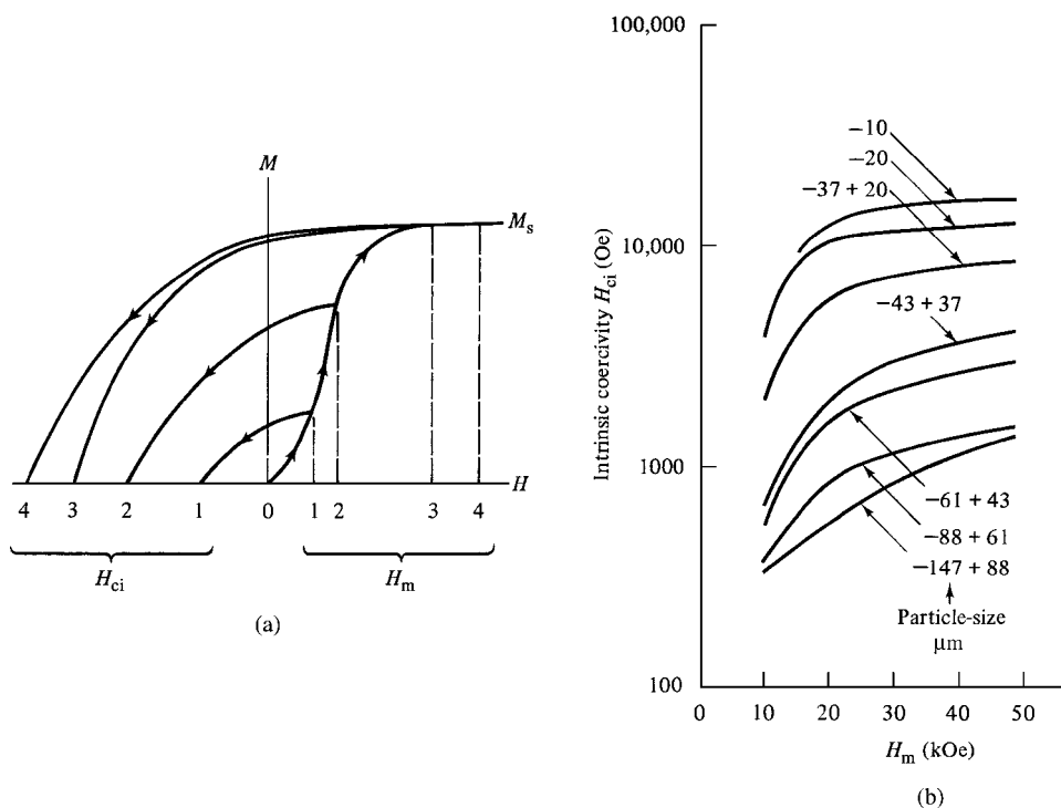
Fig. 11.15 Dependence of coercivity on maximum value H_m of magnetizing field. (a) Schematic. (b) Experimental results on aligned particles of \text{SmCo}_5 . [J. J. Becker, J. Appl. Phys. , 39 (1968) p. 1270.]
