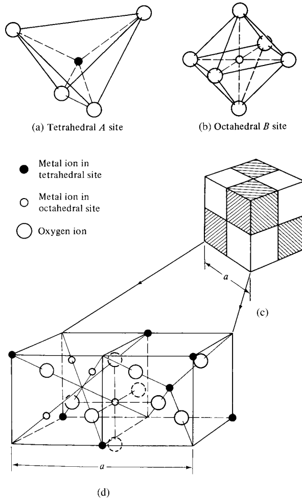
Fig. 6.2 Crystal structure of a cubic ferrite.
