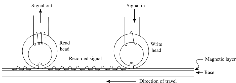
Fig. 15.1 Principle of magnetic recording.
