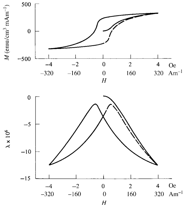
Fig. 8.25 Hysteresis in the magnetization and magnetostriction of nickel. [L. W. McKeehan, J. Franklin Inst. , 202 (1926) p. 737.]
