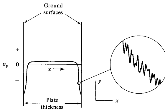
Fig. 9.30 Residual stress distribution due to grinding.
