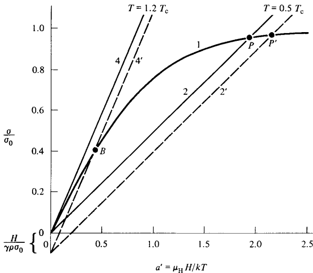
Fig. 4.8 Effects of temperature and applied field on magnetization. Curve 1 is the Brillouin function for J = \frac{1}{2} .
