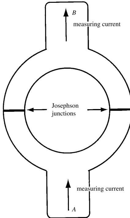
Fig. 2.19 SQUID (superconducting quantum interference device) flux sensor.
