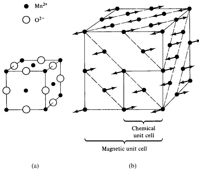
Fig. 5.16 Structure of \text{MnO} . (a) Chemical unit cell of Mn and O ions. (b) Chemical and magnetic units cells, Mn ions only.
