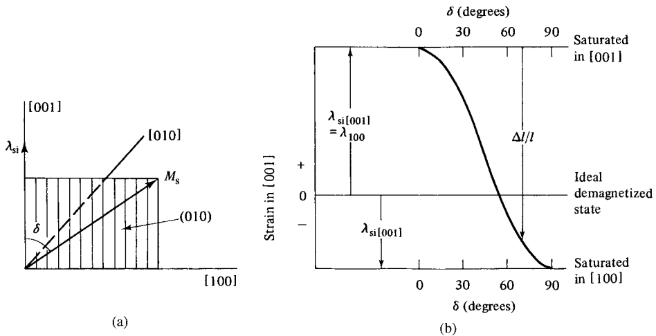
Fig. 8.3 Magnetostrictive strains in a cubic crystal with \lambda_{100} .
