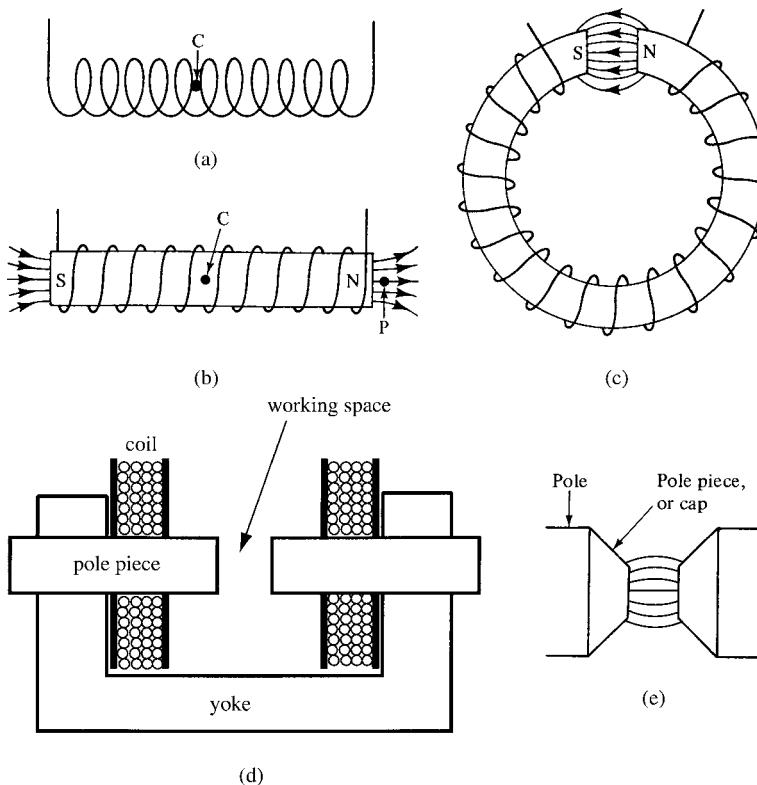
Fig. 2.9 Evolution of the electromagnet.
