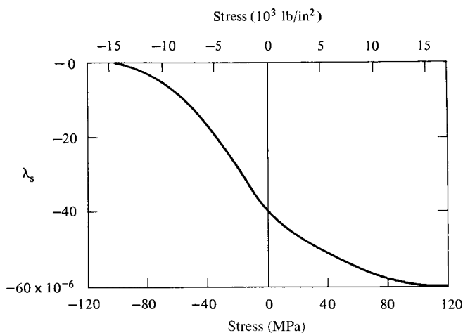
Fig. 8.23 Saturation magnetization of nickel under tension and compression. [H. Kirchner, Ann. Phys. , 27 (1936) p. 49.]
