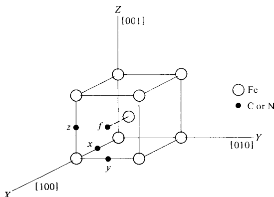
Fig. 10.9 Positions of carbon or nitrogen atoms in the unit cell of iron.
