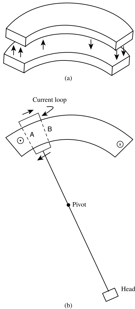
Fig. 14.19 Hard drive head positioner. (a) Magnet configuration; (b) current loop in magnet field, with head at the other end of the pivoted arm.
