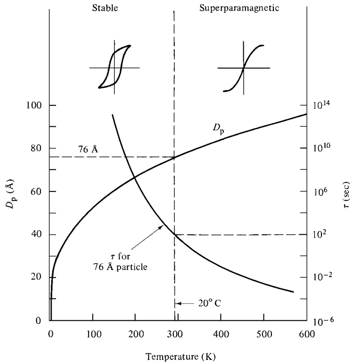
Fig. 11.19 Temperature dependence of the relaxation time \tau for spherical cobalt particles 76 Å in diameter and of the critical diameter D_p of spherical cobalt particles.
