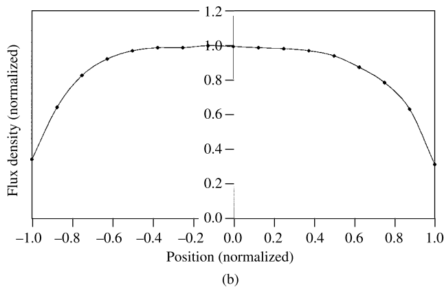
Fig. 2.23 (a) Measured flux density vs position in a steel bar magnet. (b) Same for an alnico bar magnet. The two magnets had similar length/area ratios.
