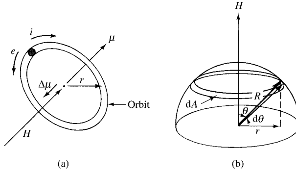
Fig. 3.2 Effect of field on orbital moment.
