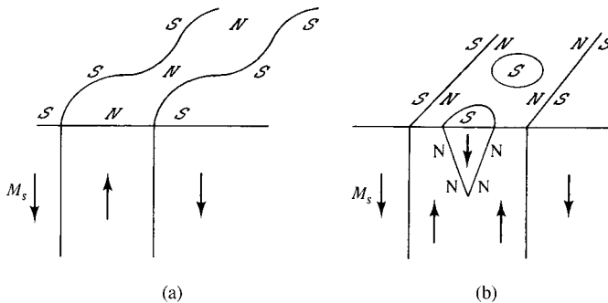
Fig. 9.17 Curved domain walls and surface spike domains.
