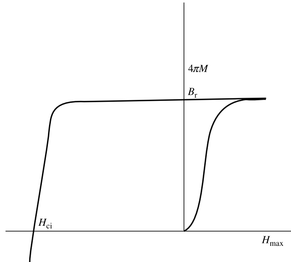
Fig. 14.12 Magnetization and demagnetization behavior of \text{SmCo}_5 (schematic).
