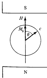
Fig. 7.9 Uniaxial disk sample in a saturating magnetic field produced by an electromagnet. c = easy axis.
