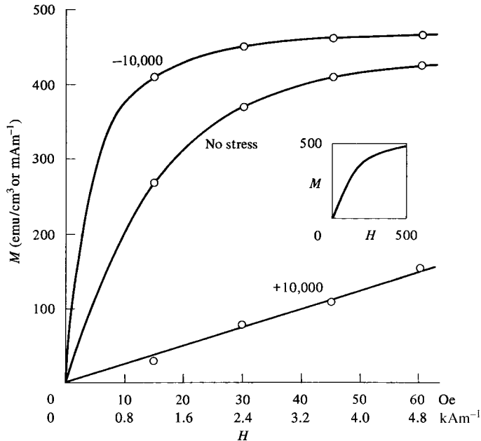
Fig. 8.16 Effect of applied tensile (+) and compressive (−) stress on the magnetization curve of polycrystalline nickel; 10,000 lb/in 2 ≈ 69 MPa. [D. K. Bagchi, unpublished.]
