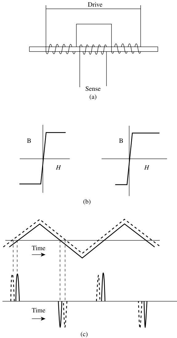
Fig. 13.24 Simple form of fluxgate magnetometer. (a) High-permeability strip or wire with drive coil and sense coil; (b) idealized hysteresis loops in zero applied field (left) and positive applied field (right); (c) upper curve is triangular current vs time in drive coil, lower curve is resulting dB/dt signal in sense coil, both on the same time axis. Solid lines correspond to zero applied field, dashed lines to small positive applied field.
