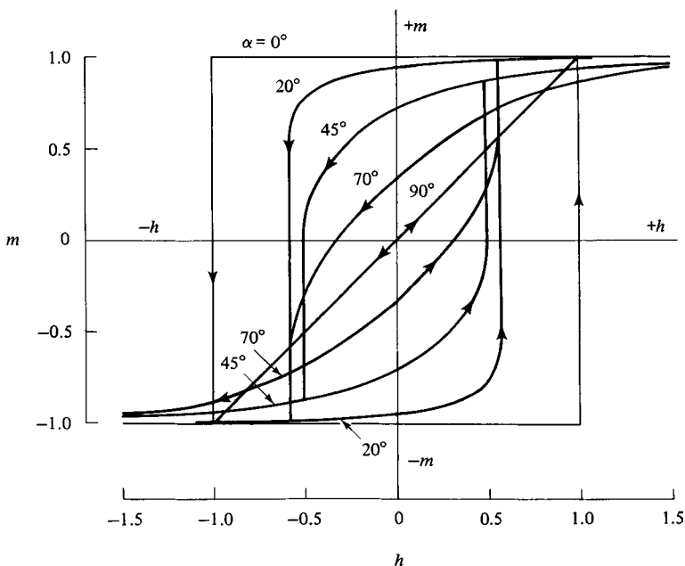
Fig. 9.36 Hysteresis loops for single domain particles with uniaxial anisotropy; \alpha is the angle between the field and the easy axis.
