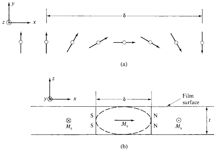
Fig. 11.31 Structure of Néel wall. (a) Section parallel to film surface. (b) Cross section of wall.
