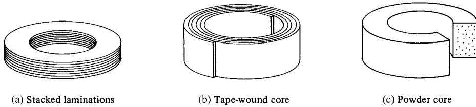
Fig. 13.21 Types of cores. The powder core has been sectioned to indicate its internal structure.
