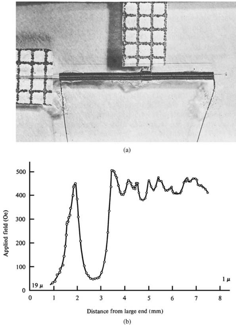
Fig. 11.14 Measurement of magnetization reversal in iron whiskers. (a) Apparatus. (b) Applied field required for reversal at various points along the length of the whisker. [R. W. DeBlois and C. P. Bean, J. Appl. Phys. , 30 (1959) p. 225S.]
