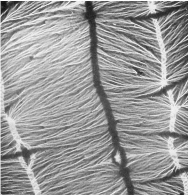
Fig. 11.38 Transmission electron micrograph of a cobalt film, 500 Å thick. [Courtesy of E. J. Torok, Sperry Rand Univac Division, St. Paul, Minnesota.]
