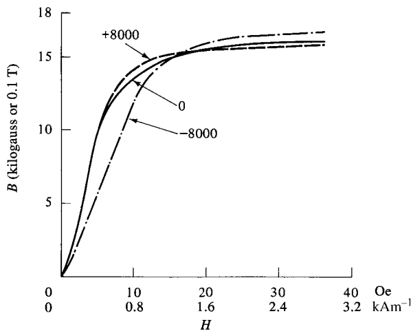
Fig. 8.18 Effects of applied tensile (+) and compressive (−) stress on the magnetization curve of iron; 8000 \text{ lb} \cdot \text{in}^2 \approx 55 \text{ MPa} .
