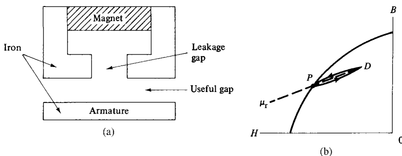
Fig. 14.8 (a) Lifting magnet. (b) Path followed on B, H curve.
