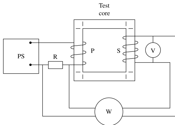
Fig. 13.6 Simplified circuit for core-loss measurement on Epstein specimens. PS = power supply, R = resistor, P = primary winding, S = secondary winding, V = voltmeter, W = wattmeter.
