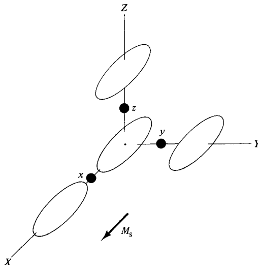
Fig. 10.11 Relation of interstitial sites x, y, z to iron atoms elongated in the magnetization direction.
