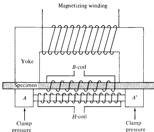
Fig. 2.43 Fahy Simplex permeameter (sketch).
