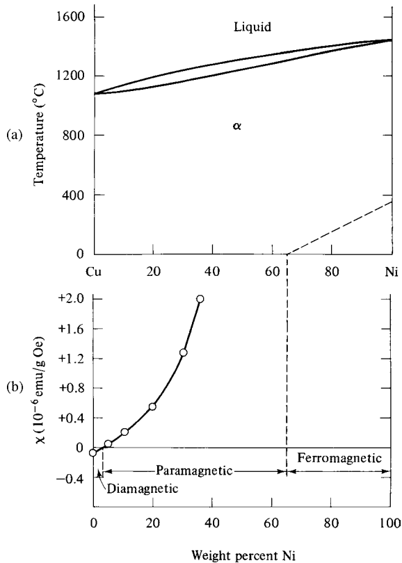
Fig. 3.11 (a) Phase diagram of the Cu–Ni system. (b) Mass susceptibility of Cu–Ni alloys at room temperature.
