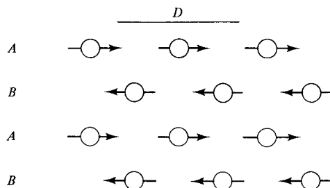
Fig. 5.2 Antiferromagnetic arrangement of A and B sublattices.
