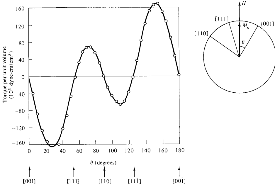
Fig. 7.15 Measured torque of a \{011\} disk of an Fe + 3.85 wt% Si alloy. The fitted curve is drawn for K_1 = 2.87 \times 10^5 erg/cm ^3 and K_2 = 1 \times 10^5 erg/cm ^3 . [R. M. Bozorth, Ferromagnetism , reprinted by IEEE Press (1993).]
