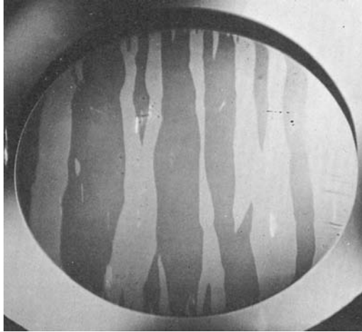
Fig. 9.13 Domains in a film of 81 permalloy observed using the Kerr effect.
