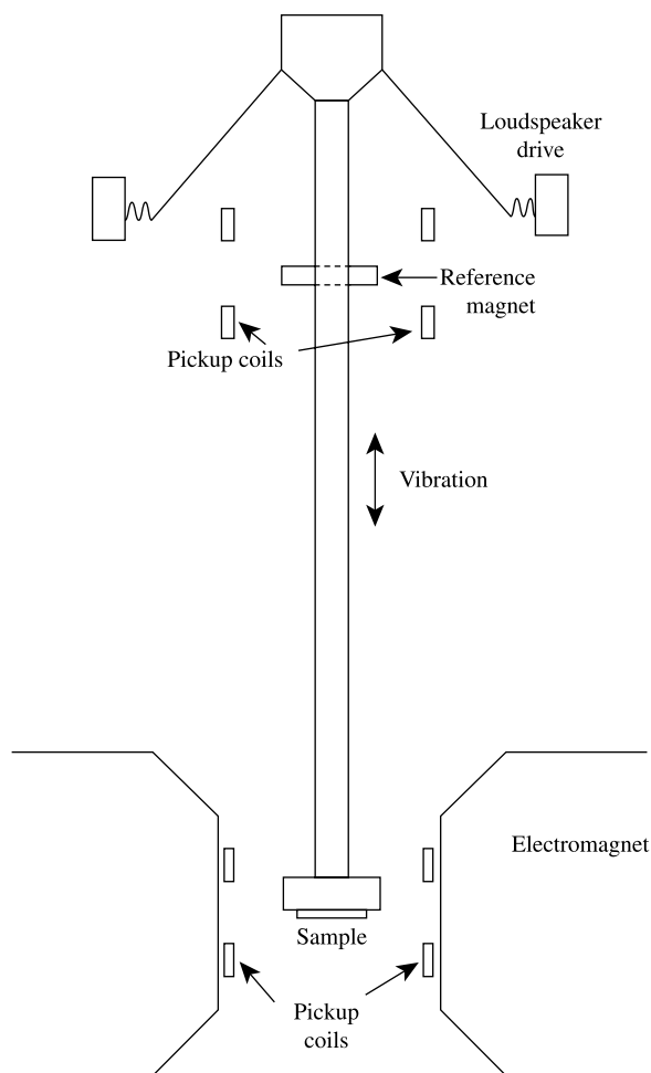
Fig. 2.37 Vibrating sample magnetometer or VSM (schematic).
