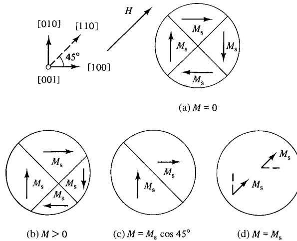
Fig. 7.4 Domain structures in a single crystal of iron (schematic). The field H is applied in the [110] direction.
