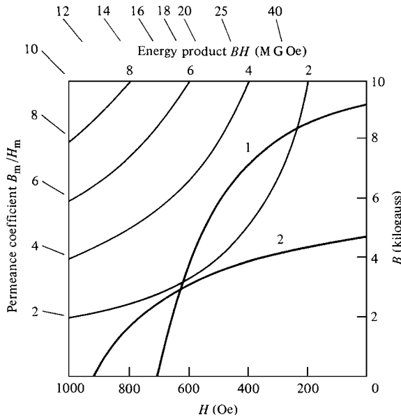
Fig. 14.4 Demagnetization curves (schematic) of two permanent magnet materials denoted 1 and 2. The graph shows also contour lines of constant ( BH ), and perimeter marks to allow values of the permeance coefficient to be drawn. Material 1 has (BH)_{max} about 3 MGOe; the value for material 2 is just below 2 MGOe.
