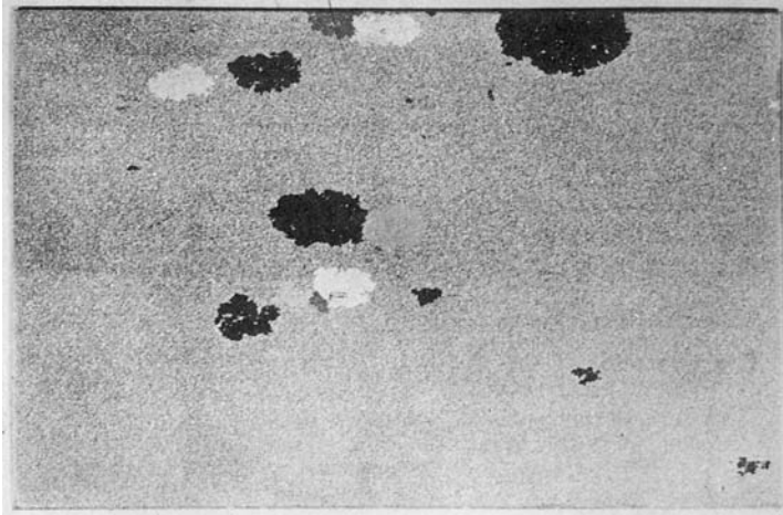
Fig. 13.13 Partial secondary recrystallization in silicon iron. A few large secondary grains are growing in a matrix of primary grains during a 900°C anneal. About actual size. [C. G. Dunn, Cold Working of Metals , ASM (1949) p. 113.]
