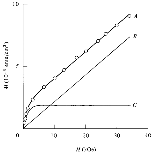
Fig. 3.12 Magnetization curve of copper containing 0.1 wt% iron (curve A). See text for meaning of curves B and C.
