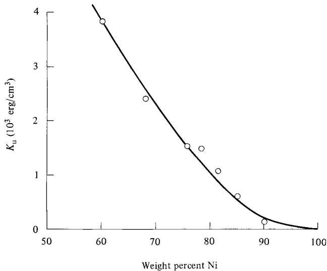
Fig. 10.5 Uniaxial anisotropy constant K_u of polycrystalline Ni–Fe alloys, cooled in a field from 600 to 80°C at 10°C/h. [S. Chikazumi and T. Oomura, J. Phys. Soc. Japan , 10 (1955) p. 842.]
