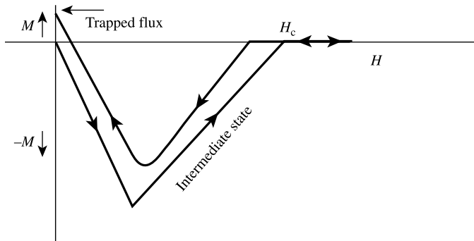
Fig. 16.3 Hysteretic behavior of a type I superconductor ( N \neq 0 ).
