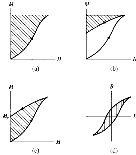
Fig. 7.23 Work done in magnetization.
