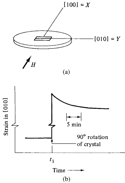
Fig. 10.10 Experiment to determine the preferred interstitial sites in iron. [After DeVries et al. Physica , 25 (1959) p. 1131.]
