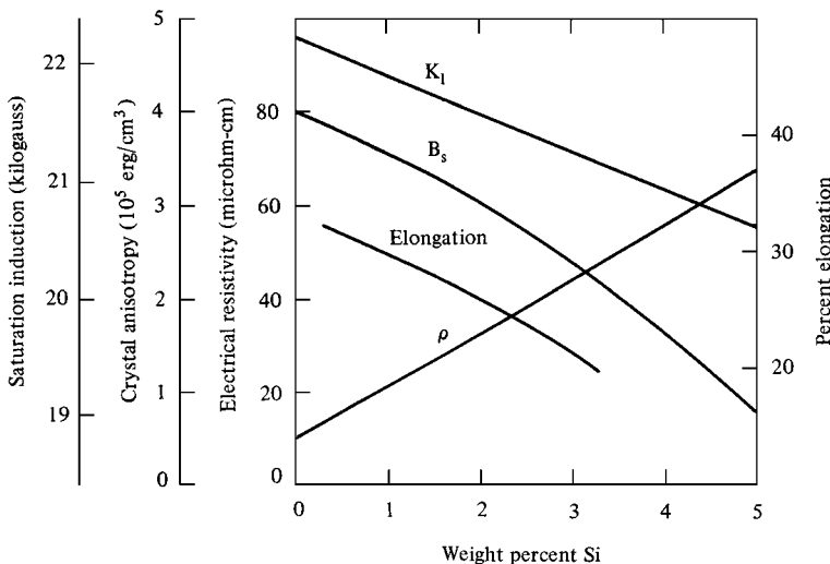
Fig. 13.12 Data on iron-silicon alloys: magnetocrystalline anisotropy constant K_1 , saturation induction B_s , electrical resistivity \rho and percentage elongation for nonoriented, polycrystalline sheet, 0.0185 inch or 0.47 mm thick.
