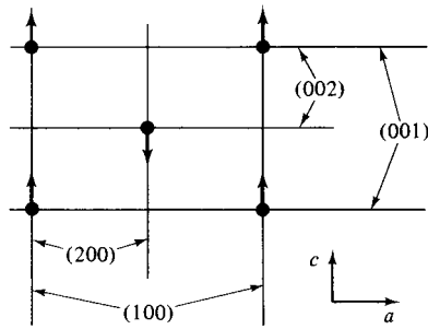
Fig. 5.15 Projection of the \text{MnF}_2 unit cell on a (010) face. Only the Mn ions are shown.
