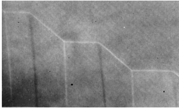
Fig. 9.11 Domain photographs of an iron foil by transmission electron microscopy, 5600 \times . [J. T. Michalak and R. C. Glenn, J. Appl. Phys. , 32 (1961) p. 1261.]
