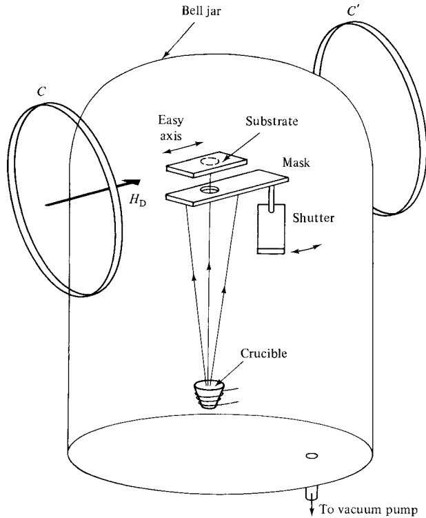
Fig. 11.29 Thin-film preparation by thermal evaporation.
