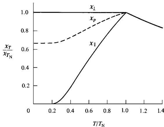
Fig. 5.7 Calculated temperature variation of the susceptibility of an antiferromagnet near and below the Néel temperature T_N . The curve of \chi_{\parallel} is calculated for J = 1 .
