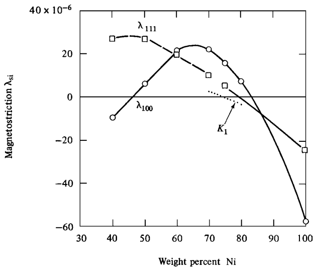
Fig. 13.19 Iron–nickel alloys. Variation of saturation magnetostriction with nickel content. See text for details. The dotted line shows K_1 from Fig. 13.18. [Data from R. C. Hall, J. Appl. Phys. , 30 (1959) p. 816.]
