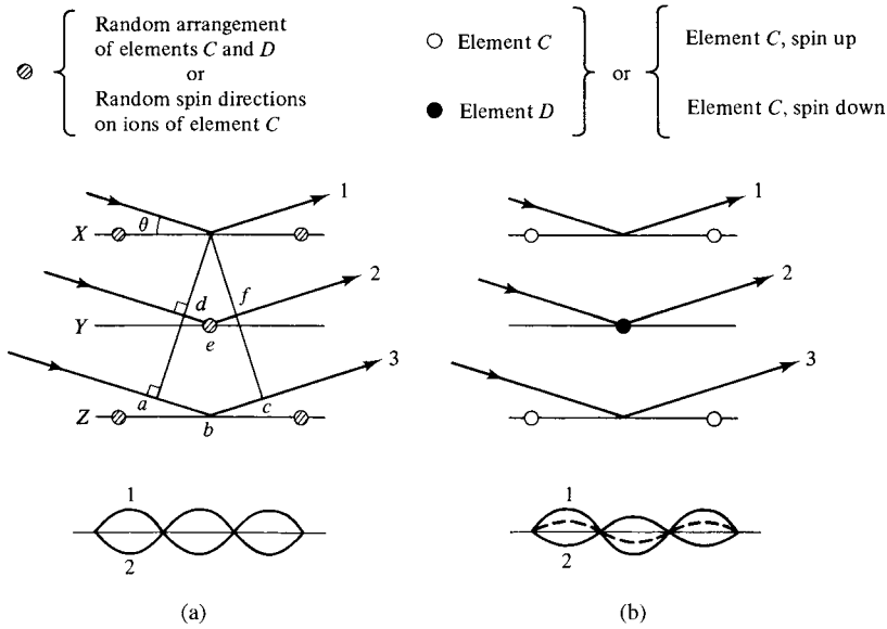
Fig. 5.11 Diffraction by (a) disordered and (b) ordered structures.
