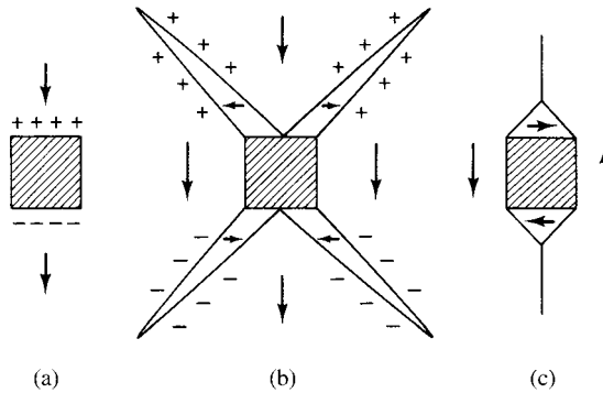
Fig. 9.27 Spike and closure domains at an inclusion., as proposed by L. Néel [ Cahiers de Physique 25 (1944) p. 21].
