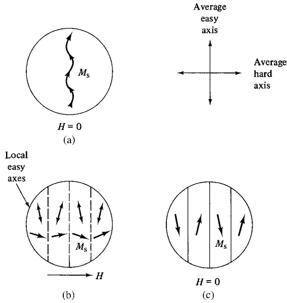
Fig. 11.37 Domain formation in a thin film after magnetization in a hard direction.
