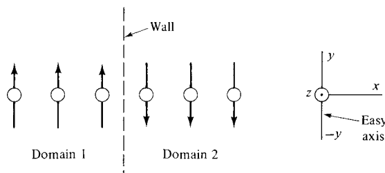
Fig. 9.1 Hypothetical 180^\circ domain wall of zero thickness.
