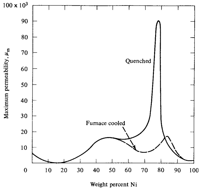
Fig. 13.20 Maximum permeabilities of iron–nickel alloys.
