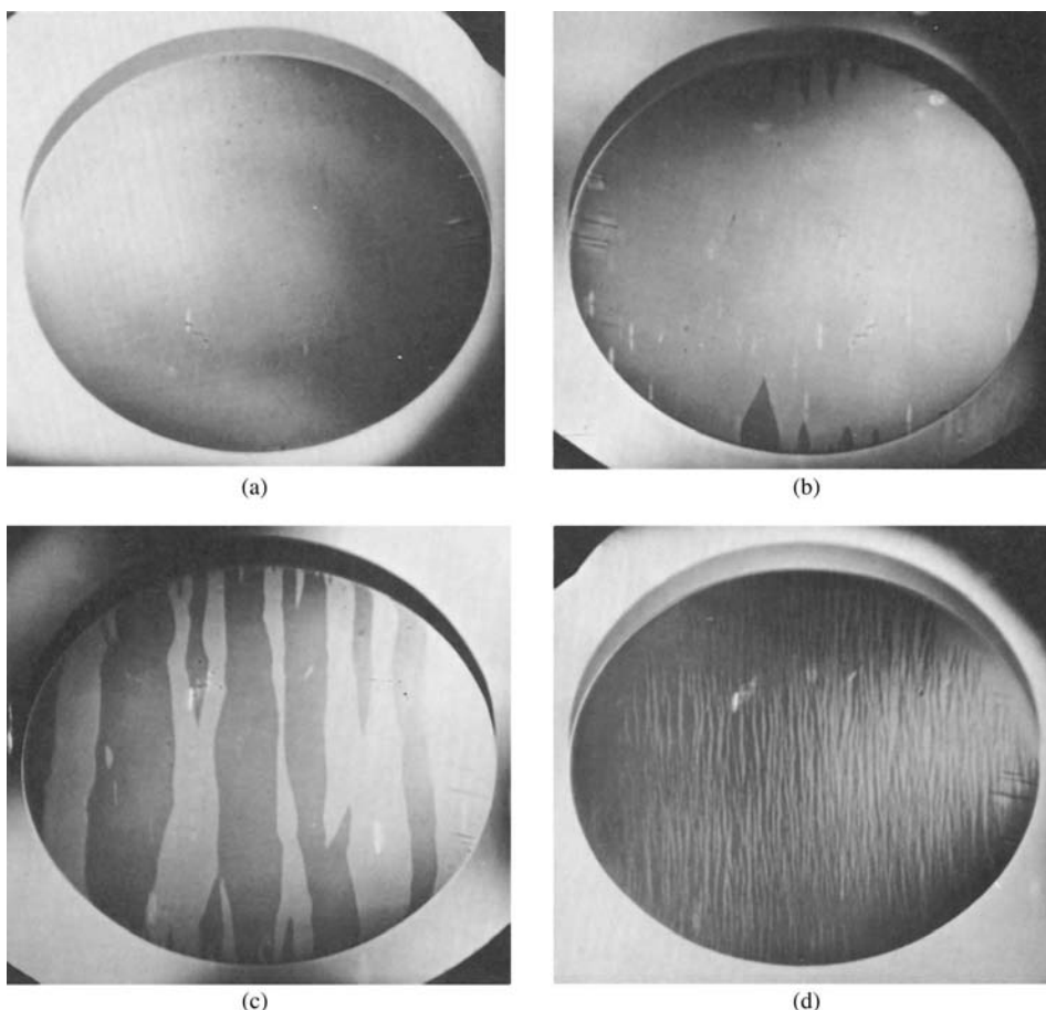
Fig. 11.36 Domains in an 81 permalloy film observed by the Kerr effect. The film is 8 mm in diameter, 2000 Å thick, and the easy axis is vertical. (a) Single-domain remanent state, H = 0 . (b) Domains nucleated at edges by a reverse easy-axis field of 0.2H_c . (c) After demagnetizing in a 60 Hz alternating field of decreasing amplitude. (d) After demagnetizing by a transverse field equal to 1.5H_K or more. [Courtesy of R. W. Olmen, Sperry Rand Univac Division, St. Paul, Minnesota.]
