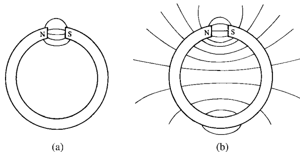
Fig. 14.5 Ring magnet showing (a) fringing and (b) leakage flux.
