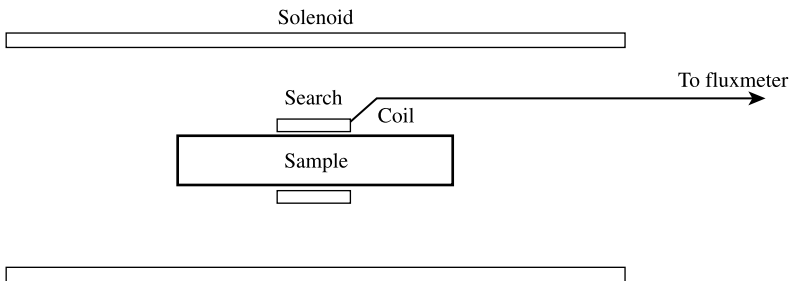
Fig. 2.35 Arrangement for measuring a rod sample in a magnetizing solenoid. Two procedures are possible: (1) solenoid current is varied continuously and fluxmeter output is recorded continuously; (2) at a series of constant solenoid current values the sample (not the search coil) is moved to a position of effectively zero field, and the fluxmeter reading is recorded. This is the extraction method. Procedure 1 measures B vs H ; procedure 2 measures M(4\pi - N) (cgs) or \mu_0M(1 - N) (SI).
