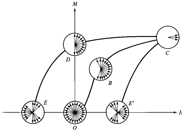
Fig. 9.43 Domain arrangements for various states of magnetization. [S. Chikazumi, Physics of Ferromagnetism , Oxford University Press (1997).]
