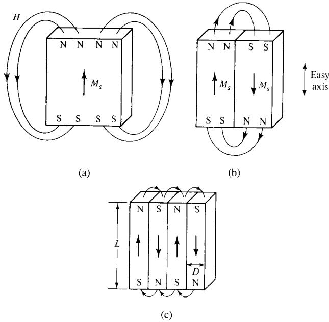
Fig. 9.16 Division of a crystal into domains. Only external H fields are shown.
