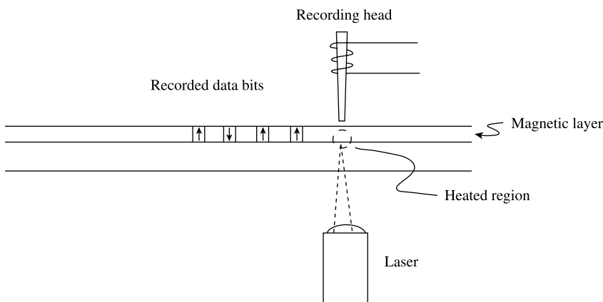
Fig. 15.8 Magneto-optic recording.
