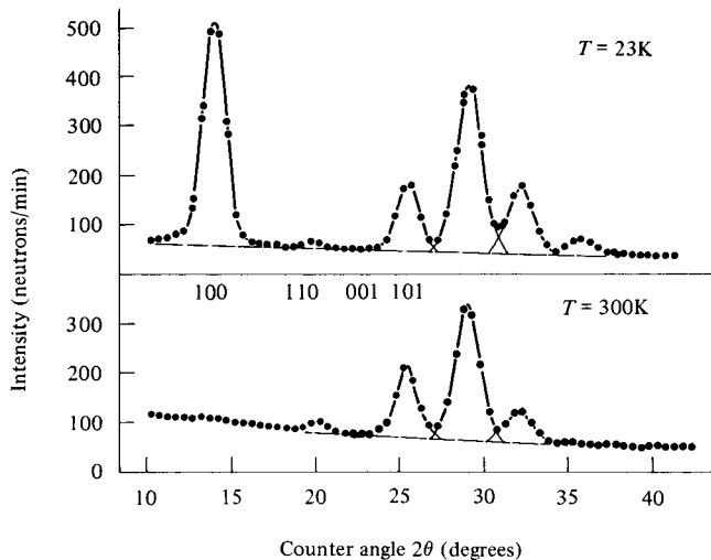
Fig. 5.14 Neutron diffraction patterns of a powder sample of \text{MnF}_2 in the paramagnetic state (300K) and in the antiferromagnetic state (23K). [R. A. Erickson, Phys. Rev. , 90 (1953) p. 779.]
