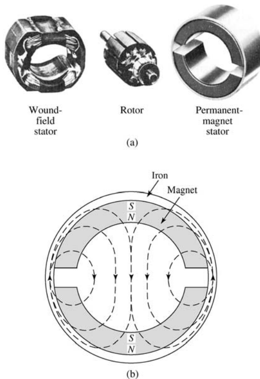
Fig. 14.18 Permanent magnet motor. (a) Comparison of a wound-field stator with a permanent magnet stator, with the same rotor; (b) the construction of the permanent magnet stator.
