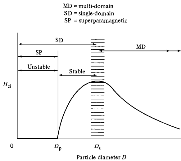
Fig. 11.2 Variation of intrinsic coercivity H_{ci} with particle diameter D (schematic).
