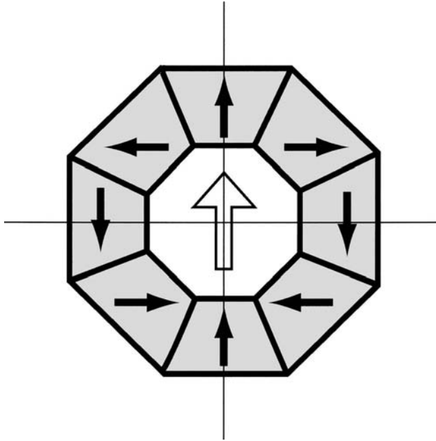
Fig. 2.13 Halbach magnet array.
