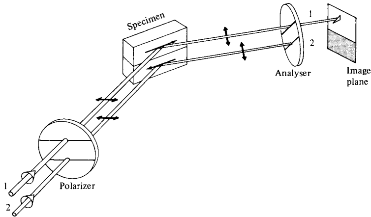
Fig. 9.12 Principle of domain observation by the Kerr effect.
