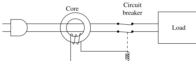
Fig. 13.22 Ground-fault interrupter circuit (schematic). If the current to the load is not equal to the current from the load, a signal voltage appears on the sensor winding and trips the circuit breaker.
