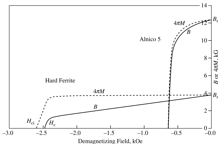
Fig. 14.6 Demagnetizing curves of alnico and hard ferrite. Solid lines are B vs H ; dotted lines are 4\pi M vs H . Note the difference between H_c and H_{ci} in the case of hard ferrite.
