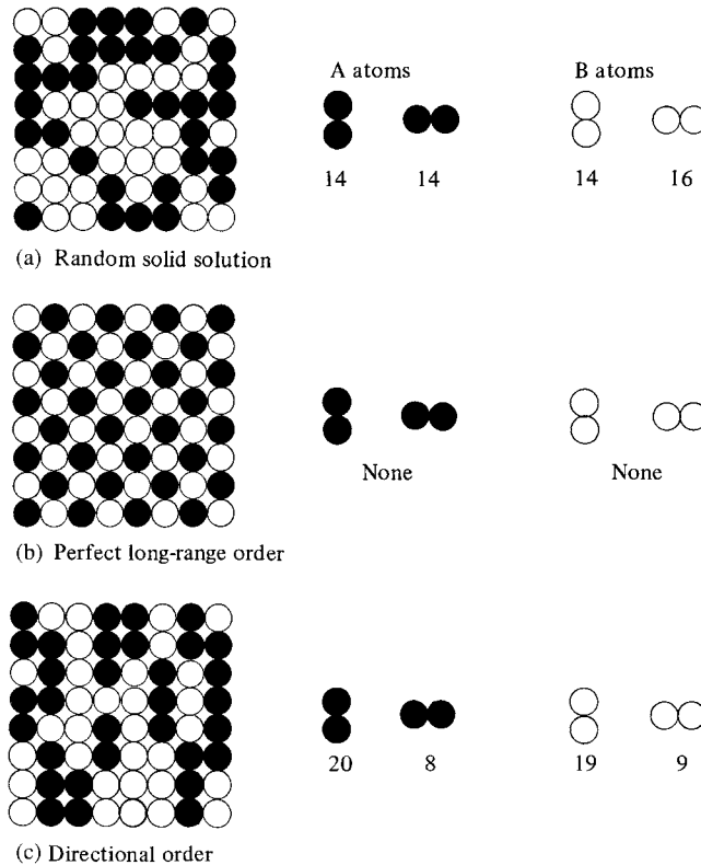
Fig. 10.4 Possible atom arrangements in a square lattice.
