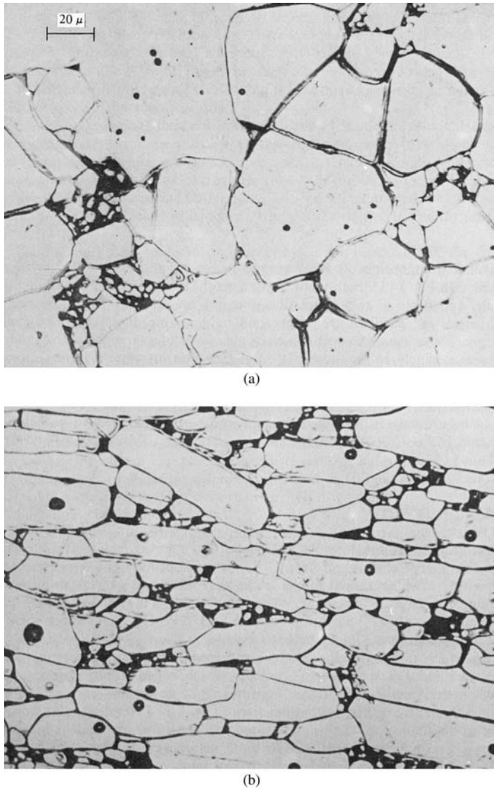
Fig. 14.11 Photomicrographs of sintered barium ferrite with oriented grains. (a) Section normal to c -axes; (b) section parallel to c -axes [J. Smit and H. P. J. Wijn, Ferrites , Wiley (1959)].
