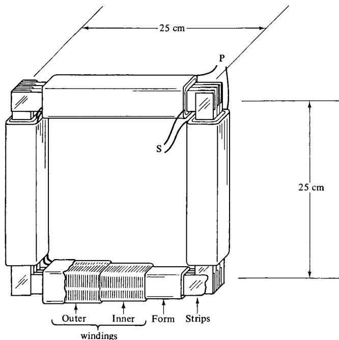
Fig. 13.5 Epstein test frame with strips inserted.
