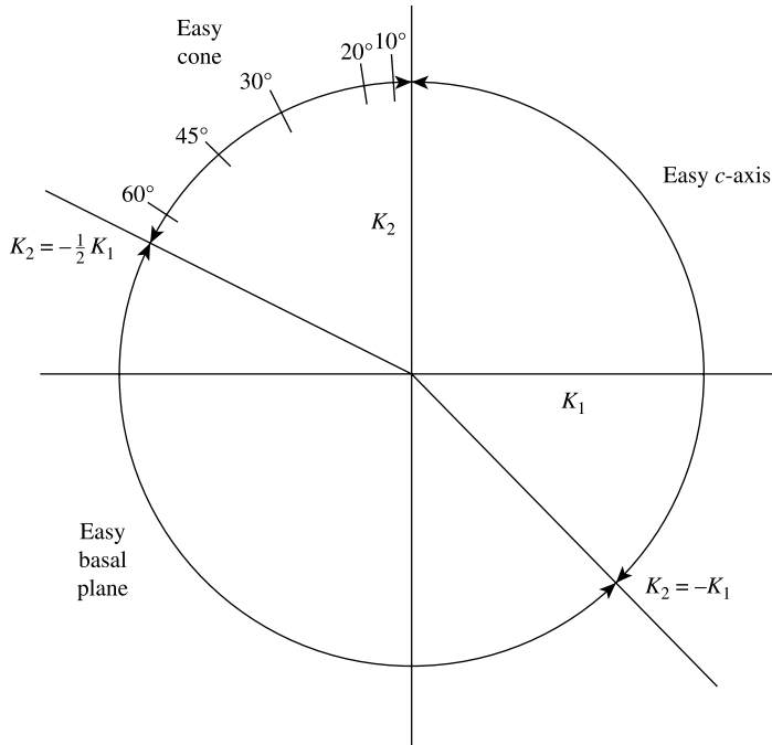
Fig. 7.7 Easy directions and planes in hexagonal crystals for all possible values of K_1 and K_2 .
