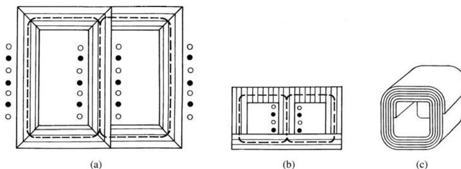
Fig. 13.16 Transformer cores. Open and closed circles represent primary and secondary windings; parallel lines denote rolling direction of sheet material.
