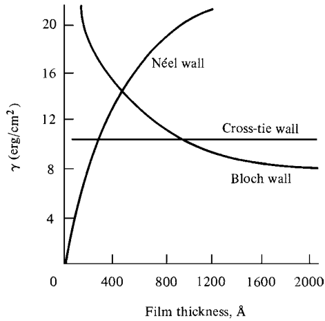
Fig. 11.32 Variation of wall energy with film thickness for various kinds of wall in 80 Permalloy, calculated for exchange constant A = 10^{-6} erg/cm, anisotropy constant K = 1500 ergs/cm 3 , bulk-wall width = 20,000 Å, and bulk-wall energy = 0.1 erg/cm 2 . [M. Prutton, Thin Ferromagnetic Films , Butterworth (1964).]
