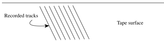
Fig. 15.3 Recorded pattern on a video tape, produced by a pair of rotating write heads.
