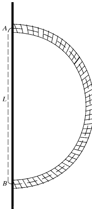
Fig. 2.18 Sketch of Chattock coil or magnetic potentiometer.
