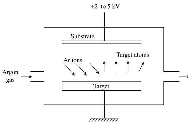
Fig. 11.28 Thin-film preparation by sputtering.
