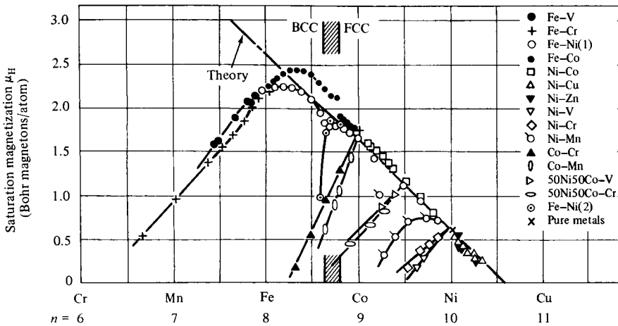
Fig. 4.22 Slater–Pauling curve: dependence of saturation magnetization of alloys on the number of (3d + 4s) electrons per atom. [S. Chikazumi, Physics of Ferromagnetism , Oxford University Press, (1997).]
