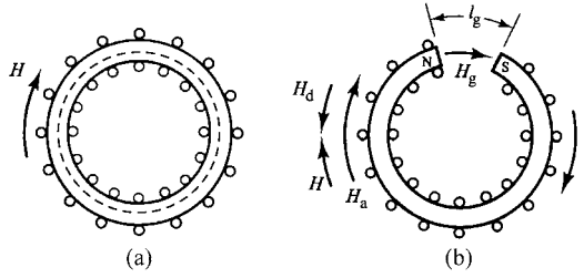
Fig. 2.42 Magnetic circuits. (a) closed, (b) open.
