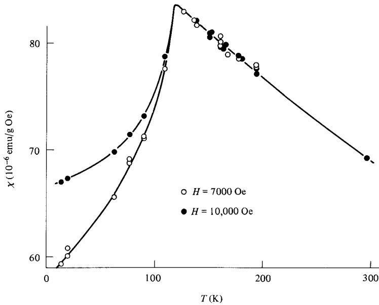
Fig. 5.8 Temperature variation of the susceptibility of MnO powder. [H. Bizette, C. F. Squire, and B. Tai, Compt. Rend. , 207 (1938) p. 449.]
