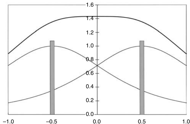
Fig. 2.3 Field distribution in Helmholtz coils. Position is specified in units of the coil radius r . The light lines show the field (normalized to unity) from the individual coils (gray bars), located at \pm 0.5 r , and the heavy line is the total field.
