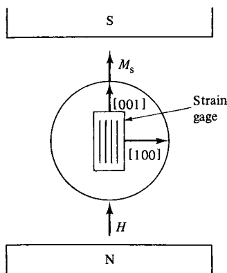
Fig. 8.4 Magnetostriction measurement on a single crystal using a strain gage.
