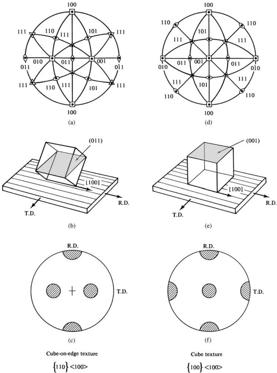
Fig. 13.14 Single-crystal projections (top), unit-cell orientations (center), and \{100\} pole figures (below). RD = rolling direction; TD = transverse direction.
