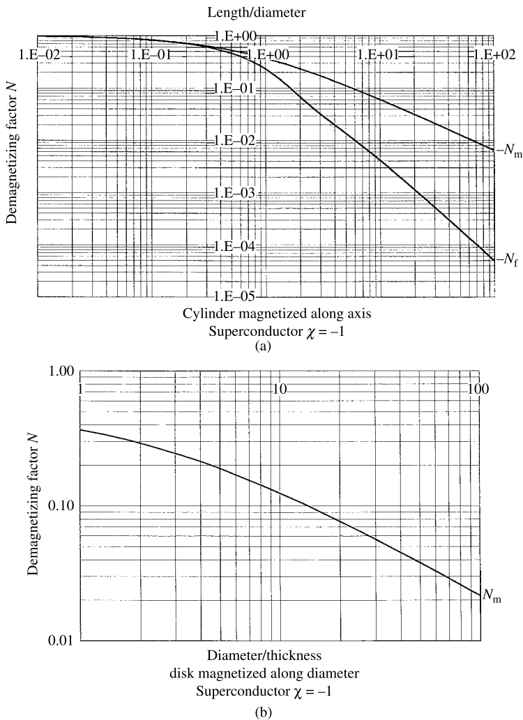
Fig. 16.9 Calculated demagnetizing factors for superconducting cylinders ( \chi = -1 ). (a) cylinder magnetized along the axis. Lower curve is fluxmetric demagnetizing factor N_f ; upper curve is magnetometric factor N_m . (b) Magnetometric factor N_m for cylinder magnetized along a diameter. Note that in (a) the x -axis is length/diameter and in (b) it is diameter/thickness.
