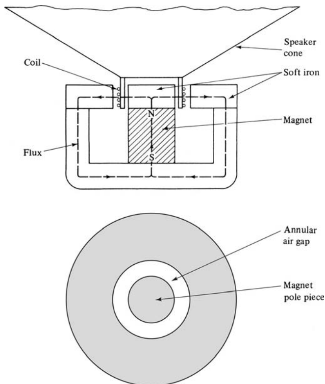
Fig. 14.17 Loudspeaker construction.
