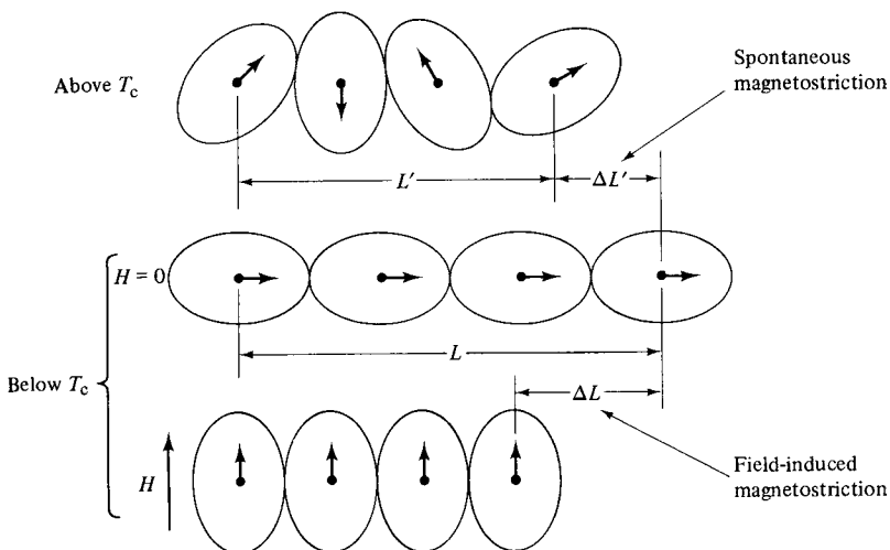
Fig. 8.15 Mechanism of magnetostriction (schematic).
