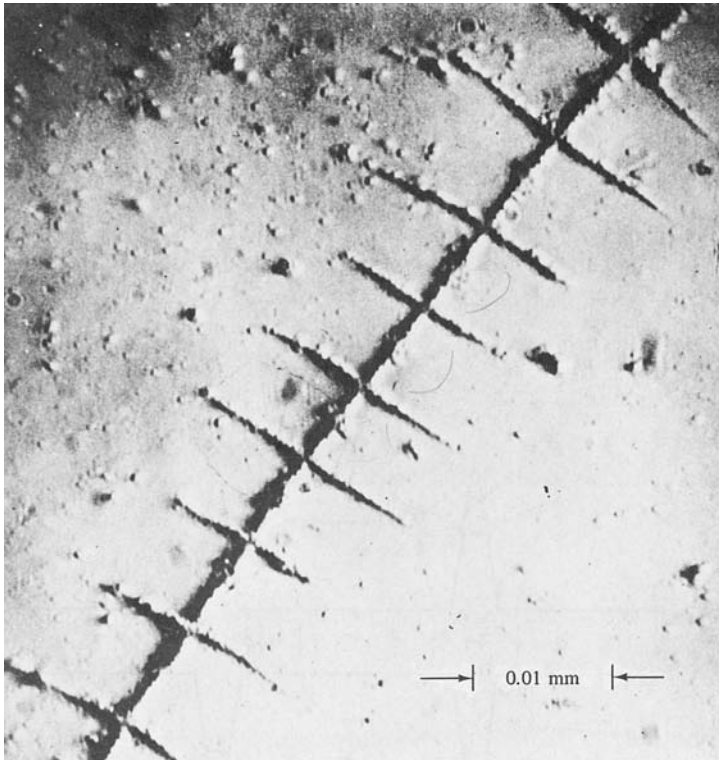
Fig. 11.33 Bitter pattern of a cross-tie wall in an 80 Permalloy film, 300 Å thick. Modified bright-field illumination. [R. M. Moon, J. Appl. Phys. , 30 (1959) p. 82S.]
