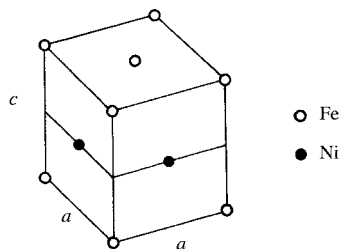
Fig. 10.15 Ordered FeNi, which has the same structure as ordered AuCu.
