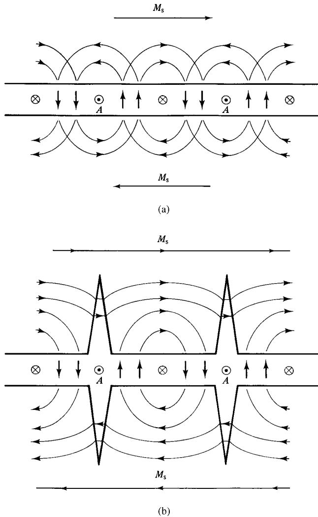
Fig. 11.34 Sections parallel to film surface of (a) hypothetical Néel wall with sections of opposite polarity, and (b) cross-tie wall.
