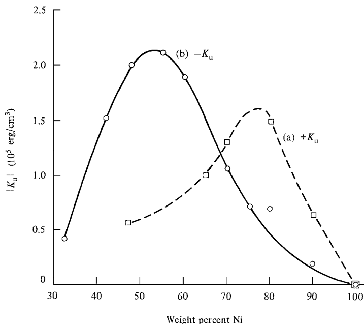
Fig. 10.12 Uniaxial anisotropy constant K_u of rolled polycrystalline Ni–Fe alloys. (a) Randomly oriented grains rolled to 33% reduction in thickness. (b) Cube-texture material rolled to 55% reduction. [After G. W. Rathenau and J. L. Snoek, Physica , 8 (1941) p. 555.]
