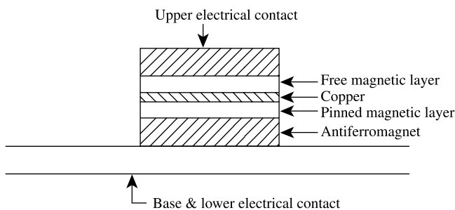
Fig. 15.5 Basic structure of a spin valve.
