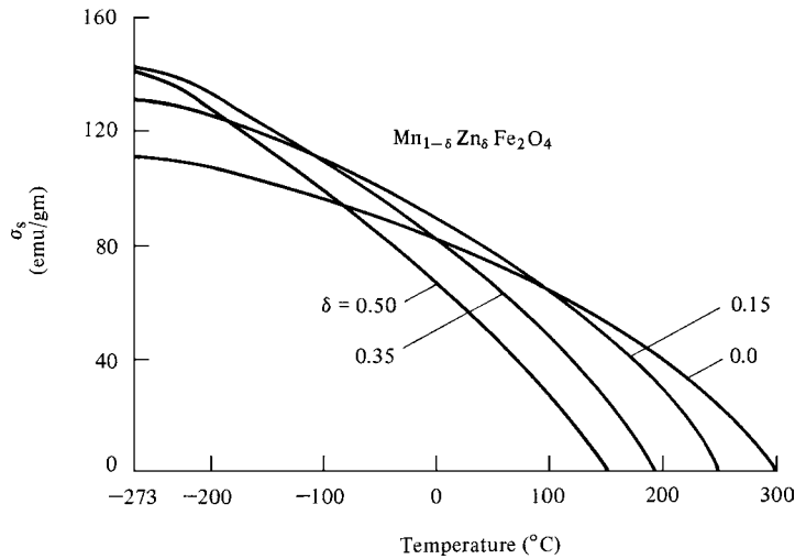
Fig. 13.26 Variation with temperature of the saturation magnetization \sigma_s of Mn-Zn ferrites.
