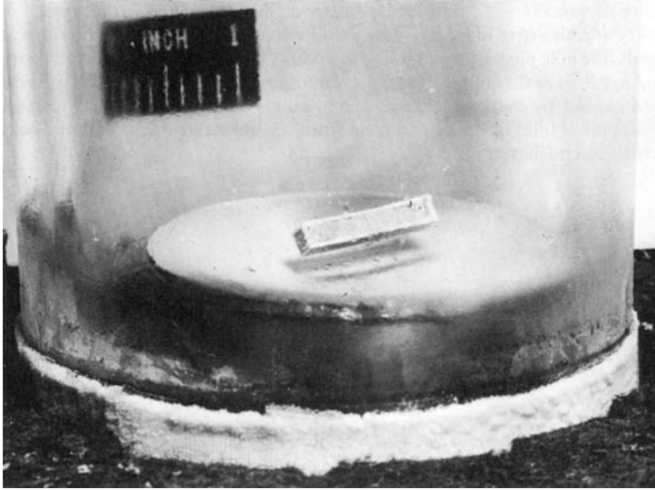
Fig. 14.22 Bar magnet suspended over a superconducting plate.
