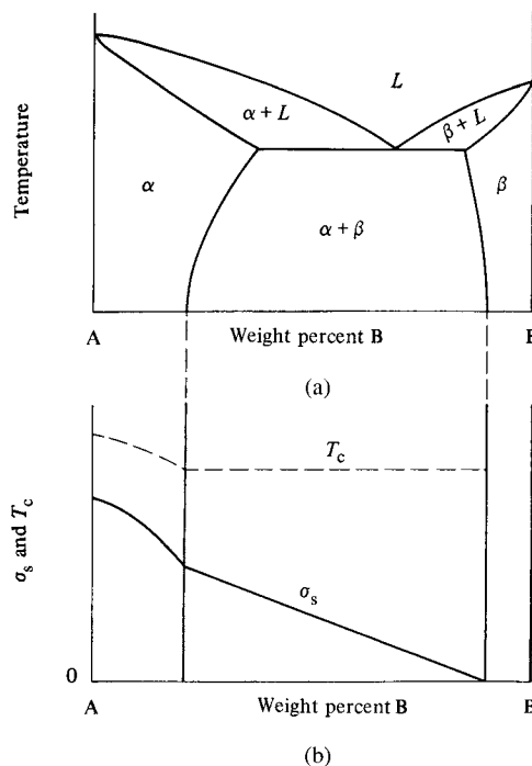
Fig. 4.20 (a) Hypothetical phase diagram of A–B alloys. Element A is ferromagnetic, B is paramagnetic. (b) Variation of \sigma_s and T_c with composition.
