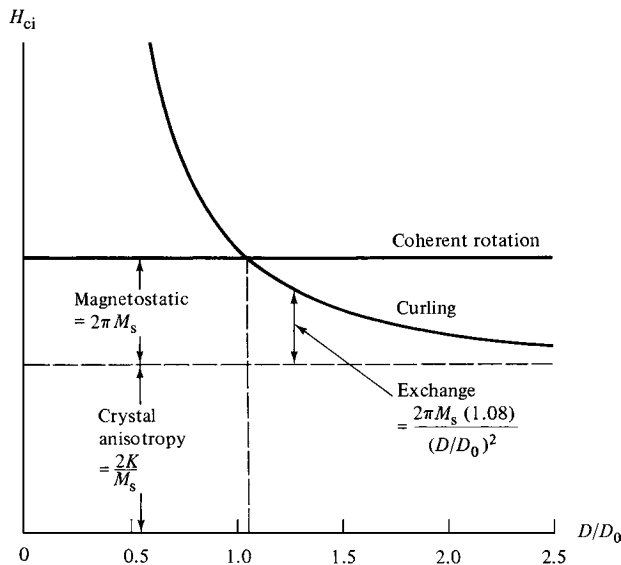
Fig. 11.10 Calculated coercivities, with the effect of crystal anisotropy included, for coherent and curling reversals in an infinite cylinder as a function of the reduced diameter D/D_0 . [After W. F. Brown, Magnetostatic Principles in Ferromagnetism , North Holland (1962).]
