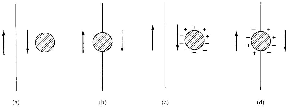
Fig. 9.26 Interaction of domain wall with inclusion.
