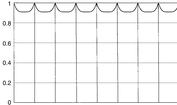
Fig. 13.3 Calculated relative flux amplitude in a stack of insulated sheets, each 0.75 mm thick, for the same conditions as in Fig. 13.2.
