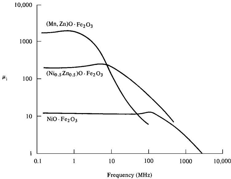
Fig. 13.28 Variation of initial permeability \mu_i with frequency for three ferrites.
