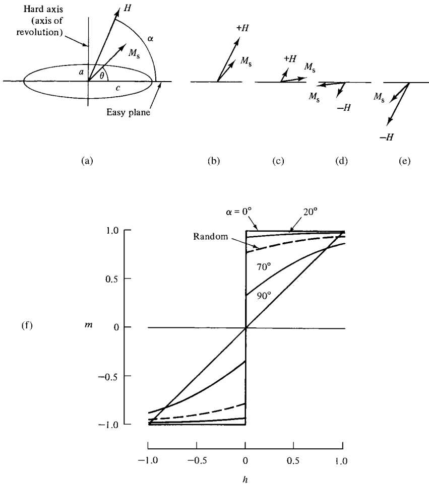
Fig. 9.38 Hysteresis behavior for planetary (oblate) spheroids.
