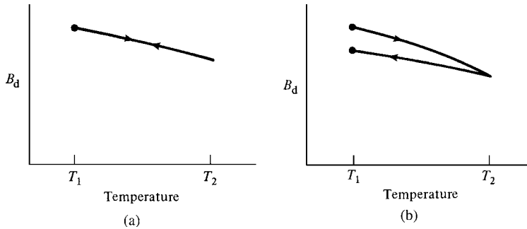
Fig. 14.16 Effects of increased temperature on the induction at the operating point. (a) Reversible; (b) irreversible.
