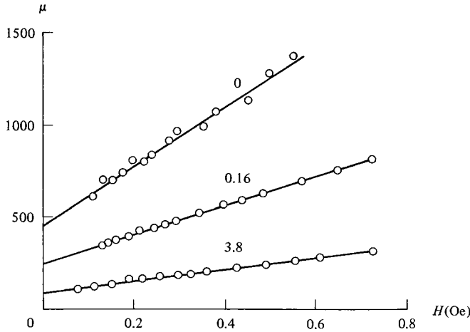
Fig. 9.40 Permeability \mu vs field strength in the Rayleigh region for iron with varying degrees of cold work. Numbers on curves are degree of plastic elongation, in percent. [R. M. Rusak, Ph.D. thesis, University of Notre Dame, South Bend, Indiana.]
