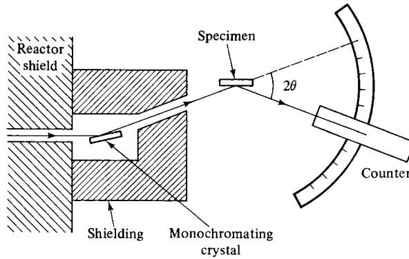
Fig. 5.13 Neutron diffractometer (schematic).
