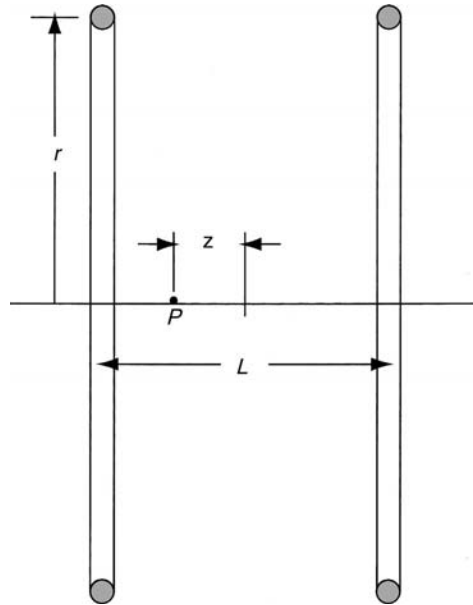
Fig. 2.2 Helmholtz coils. The spacing between coils L is equal to the coil radius r .
