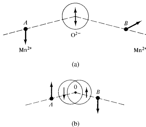
Fig. 5.19 Superexchange.
