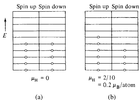
Fig. 4.17 Energy bands with (a) balanced and (b) unbalanced spins.
