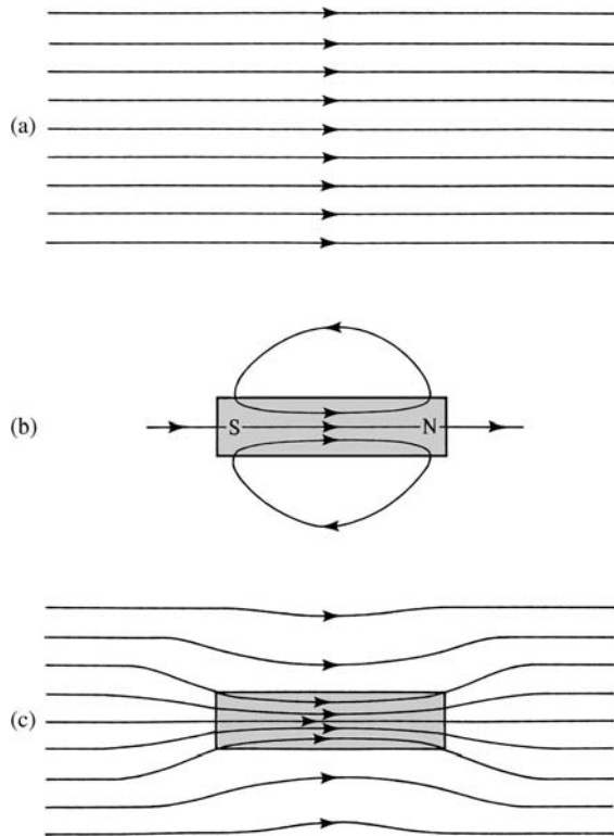
Fig. 2.24 Result of placing a magnetized body in an originally uniform field.
