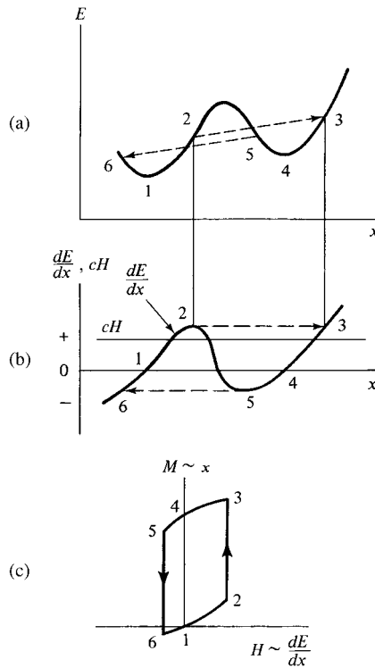
Fig. 9.34 Reversible and irreversible domain wall motion.
