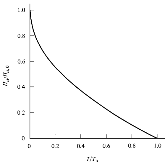
Fig. 11.21 Theoretical temperature dependence of the coercivity of single-domain fine particles. T_B = blocking temperature.
