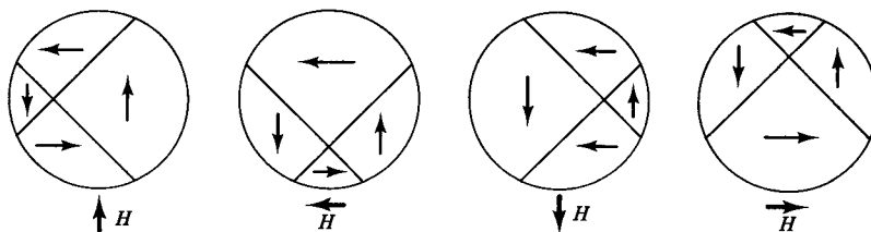
Fig. 13.8 Wall motion in a rotating field (schematic).
