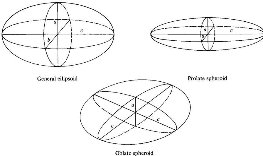
Fig. 2.27 Ellipsoids.
