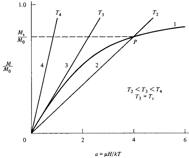
Fig. 4.4 Effect of temperature on the value of spontaneous magnetization. Curve 1 is the Langevin function.
