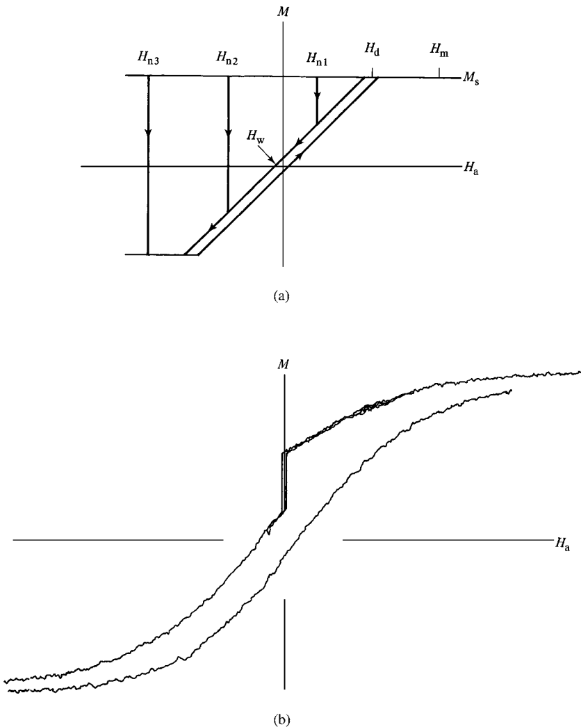
Fig. 11.16 Hysteresis loops of a single particle. (a) Theoretical. (b) Observed for a particle of \text{SmCo}_5 . [J. J. Becker, IEEE Trans. Mag. , 5 (1969) p. 211.]
