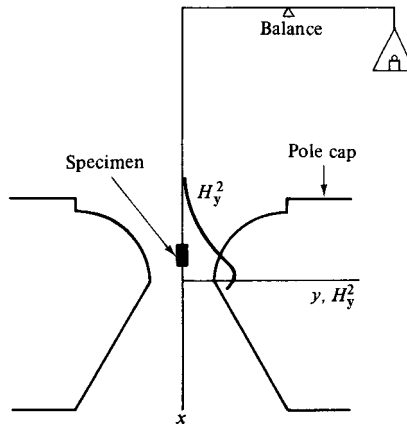
Fig. 2.47 Curie method for measurement of susceptibility.
