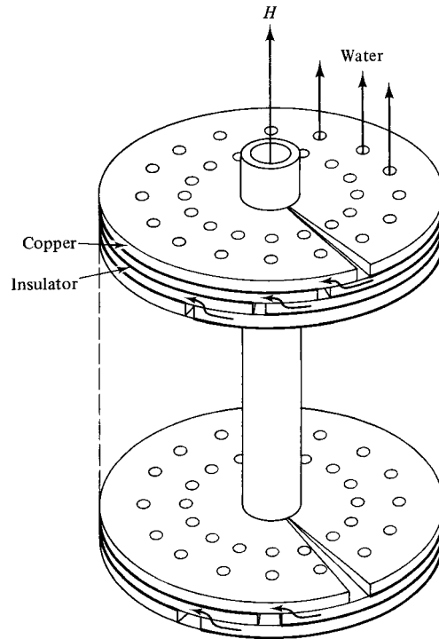
Fig. 2.5 Sketch of a Bitter magnet solenoid. Arrows indicate the current path from one disk to another.
