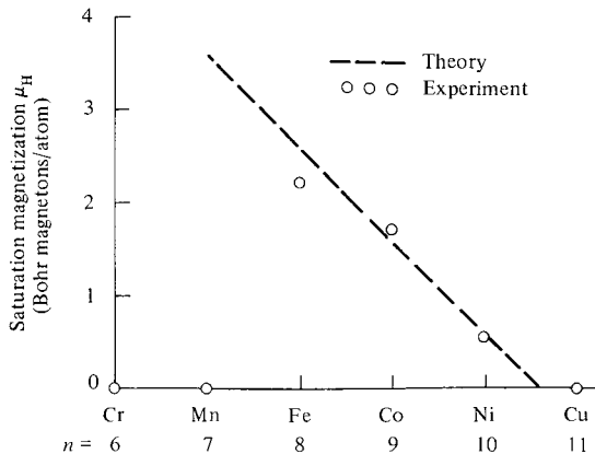
Fig. 4.18 Observed and calculated dependence of the saturation magnetization on the number n of ( 3d and 4s ) electrons per atom.
