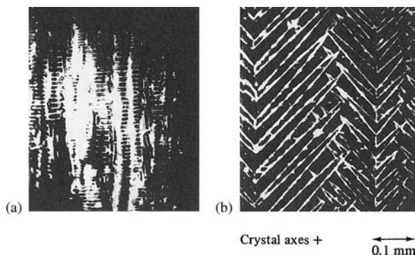
Fig. 9.9 Powder patterns on a single crystal of Fe + 3.8% Si, using dark-field illumination. (a) after mechanical polishing, (b) after electropolishing. The area viewed is about 0.5 \times 0.45 mm.
