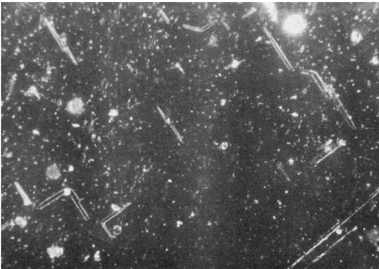
Fig. 9.28 Spike domains at inclusions in an Fe + 3% Si crystal.
