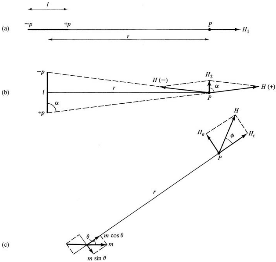
Fig. A1.1 Fields of dipoles.
