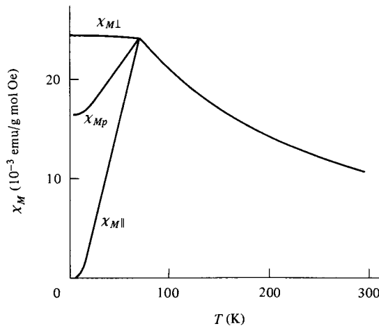
Fig. 5.9 Temperature variation of the molar susceptibility of \text{MnF}_2 . The central curve (below T_N ) is for a powder sample, and the other two curves are for a single crystal. [H. Bizette and B. Tai, Compt. Rend. , 238 (1954) p. 1575.]
