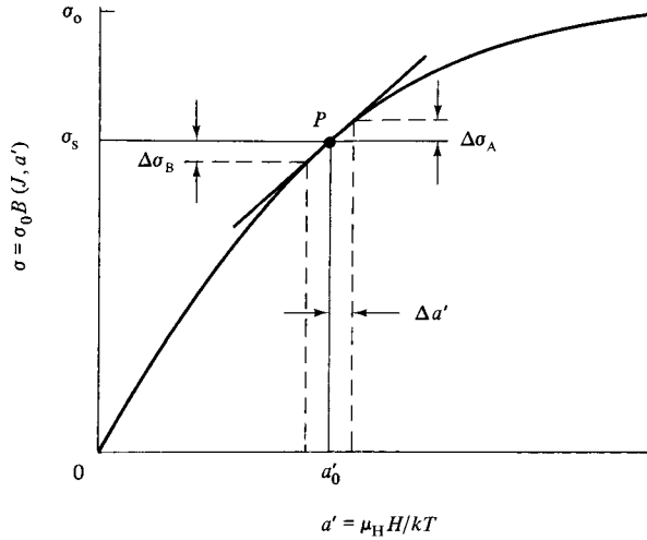
Fig. 5.6 Magnetization changes when the field is applied parallel to the spin axis.
