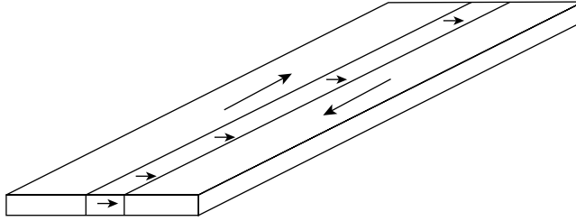
Fig. 9.7 Néel wall in thin sample. Free poles appear along the surface of the wall, but not at the sample surface.
