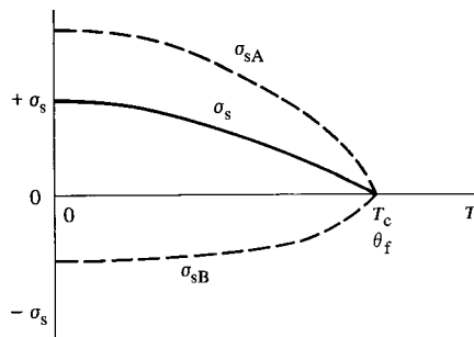
Fig. 6.8 Spontaneous magnetizations of the A and B sublattices, and the resultant saturation magnetization \sigma_s , for a typical cubic ferrimagnet (schematic).
