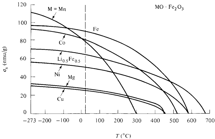
Fig. 6.11 Saturation magnetization vs temperature for several cubic ferrimagnets. [Data for Figs 6.11 and 6.13 from J. Smit and H. P. J. Wijn, Ferrites , Wiley (1959).]
