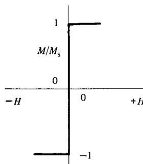
Fig. 7.18 Idealized hysteresis loop of a crystal measured parallel to an easy axis.
