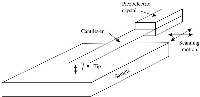
Fig. 9.14 Scanning probe microscope.
