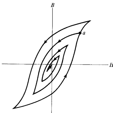
Fig. 1.16 Demagnetization by cycling with decreasing field amplitude.
