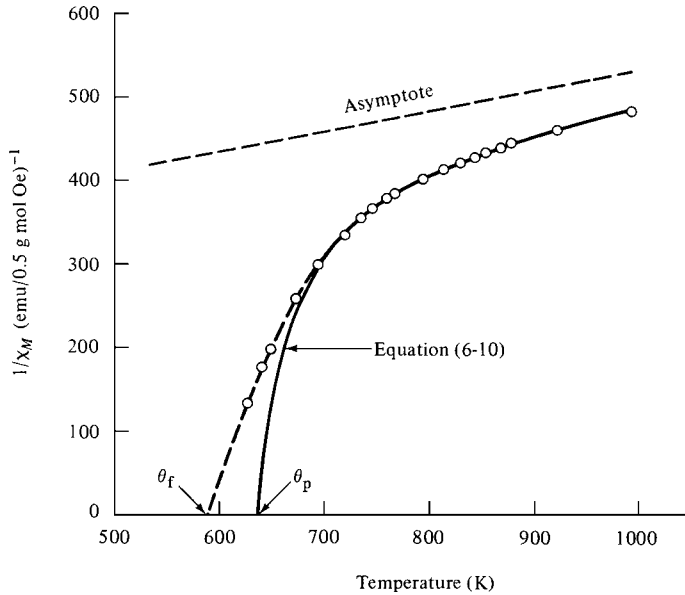
Fig. 6.7 Reciprocal susceptibility vs. temperature for Mn ferrite. Here \chi_M refers to a half molecule of ferrite, i.e., to one mol of \text{Fe}^{3+} .
