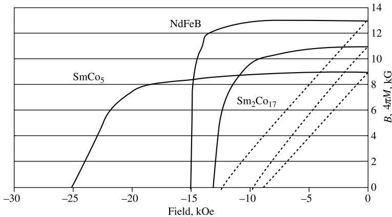
Fig. 14.13 Demagnetization curves of typical rare-earth permanent magnets.
