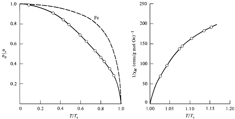
Fig. 6.1 Temperature dependence of magnetic properties of a typical ferrimagnet ( \text{NiO}\cdot\text{Fe}_2\text{O}_3 ). Left-hand figure shows the fractional saturation magnetization per unit mass \sigma_s/\sigma_0 in the ferrimagnetic region and the right-hand figure shows the reciprocal susceptibility (per mole) in the paramagnetic region. The dashed curve in the left-hand figure is the corresponding data for metallic iron.
