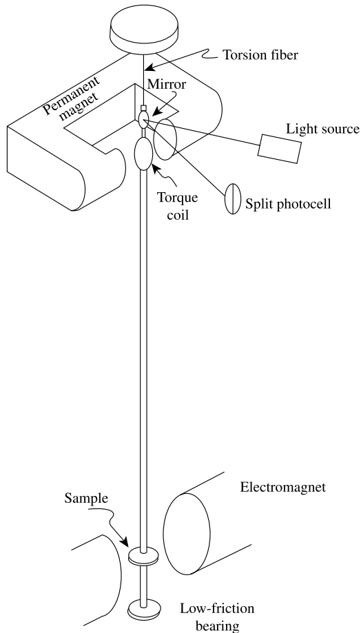
Fig. 7.17 Automatic recording torque magnetometer.
