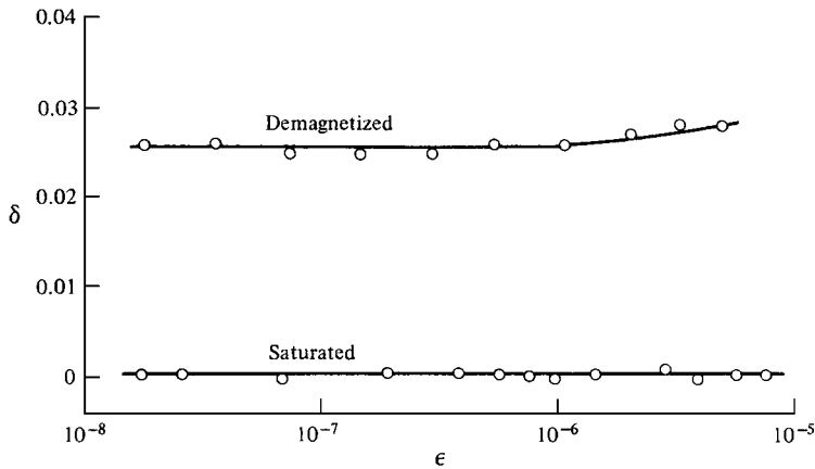
Fig. 12.16 Damping \delta (logarithmic decrement) as a function of strain amplitude \epsilon in a nickel single-crystal rod with a \langle 100 \rangle axis. Room temperature. Vibrated in the longitudinal mode at 50 kHz. [H. Ganganna, N. F. Fiore, and B. D. Cullity, J. Appl. Phys. , 42 (1971) p. 5792.]
