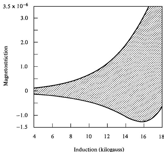
Fig. 13.17 Limits of static longitudinal magnetostriction as a function of induction for several grades and thicknesses of grain-oriented silicon steel sheet. Data from U.S. Steel.
