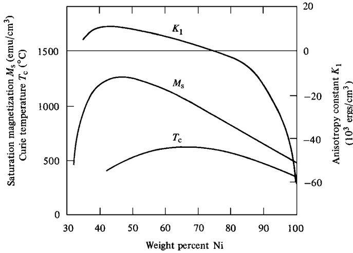
Fig. 13.18 Iron–nickel alloys. Variation with nickel content of saturation magnetization M_s , Curie temperature T_c , and magnetocrystalline anisotropy K_1 (quenched alloys). [R. M. Bozorth, Ferromagnetism , reprinted by IEEE Press (1993).]
