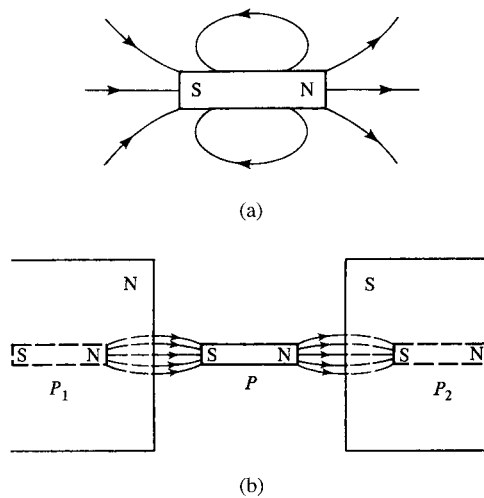
Fig. 2.40 Image effect. (a) field due to magnetized sample in empty space; (b) field due to magnetized sample placed between two soft iron pole pieces.
