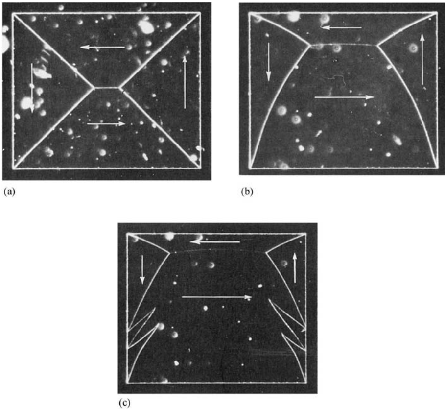
Fig. 9.21 Wall motion in a Ni-Co alloy platelet 165 \mu\text{m} across. Bitter patterns, dark field illumination.
