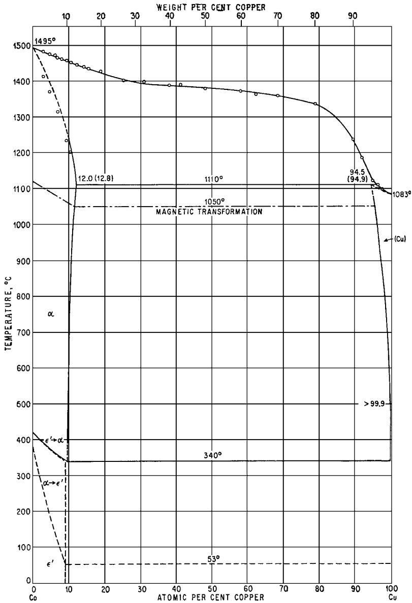
Fig. 11.22 Copper-cobalt equilibrium diagram (ASM Handbook).
