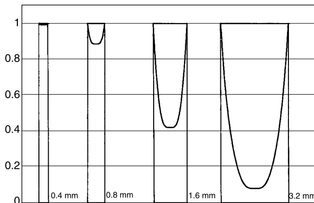
Fig. 13.2 Calculated amplitude of alternating flux in transformer steel sheets of various thicknesses as a fraction of the value at the surface. Frequency = 60 Hz, skin depth \delta = 0.5 mm, sheet thicknesses as indicated.
