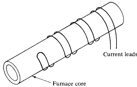
Fig. 2.49 Noninductive, or bifilar, winding.
