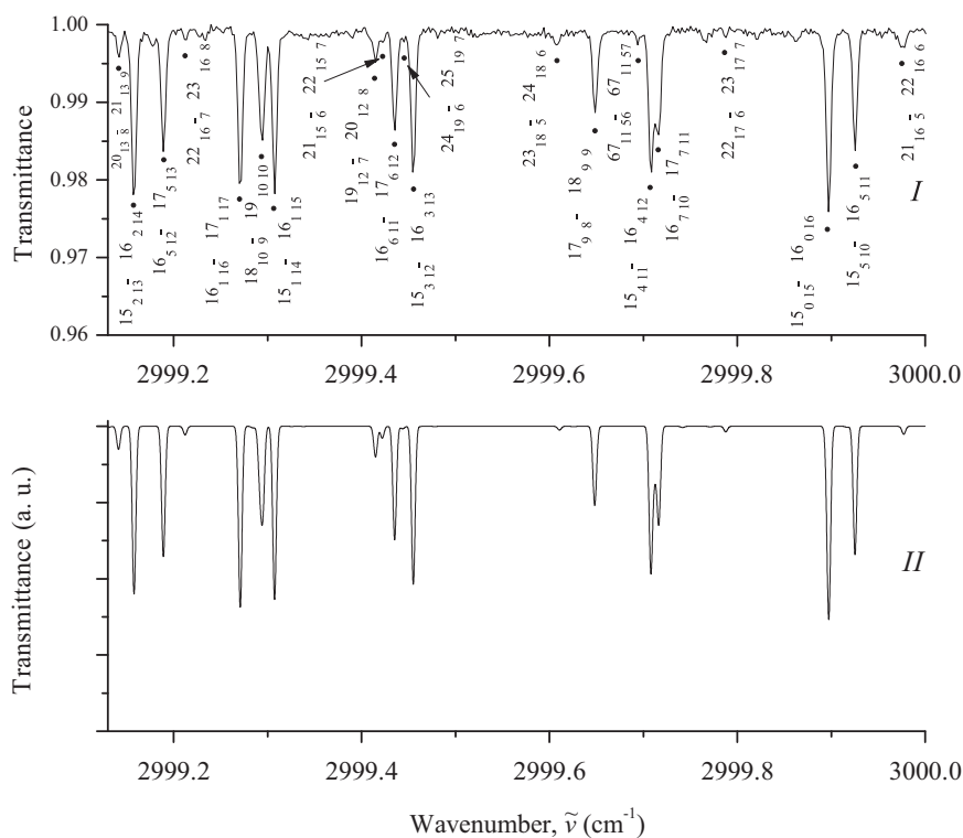
Fig. 2. Small portion of the high resolution spectrum of \text{SO}_2 in the region of the P-branch of the \nu_1 + \nu_2 + \nu_3 band (upper part). Experimental conditions: absorption path length is 163.2 m; sample pressure is 111 Pa; room temperature; registration time is 80.5 h. The simulated spectrum is shown in the lower part of the figure.
