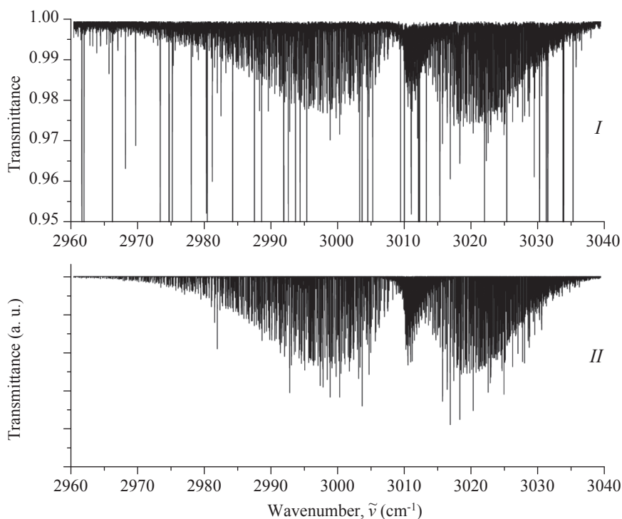
Fig. 1. Survey spectrum of \text{SO}_2 in the region of the weak \nu_1 + \nu_2 + \nu_3 band. Experimental conditions: absorption path length is 163.2 m; sample pressure is 111 Pa; room temperature; registration time is 80.5 h. The simulated spectrum is shown in the lower part of the figure.
