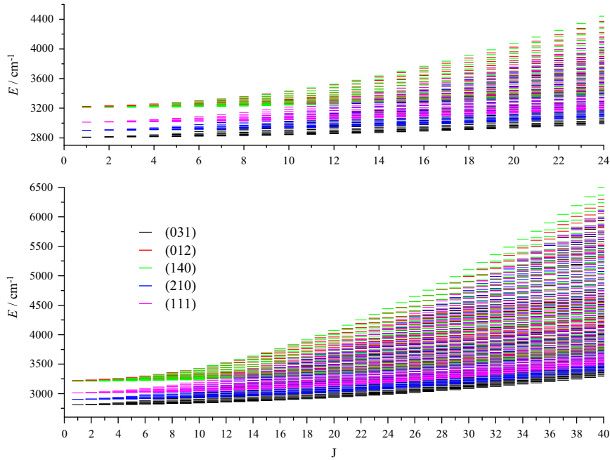
Fig. 3. Diagram of ro-vibrational energy levels of the (111), (210), (012), (140), and (031) vibrational states of SO 2 as functions of the rotational quantum number J . Different colors indicate ro-vibrational energy levels belonging to different vibrational states. (For interpretation of the references to color in this figure caption, the reader is referred to the web version of this paper.)
