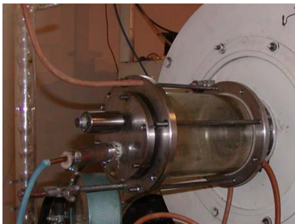
Fig. 5. Plasma chemical reactor with a volume of 6 litres
