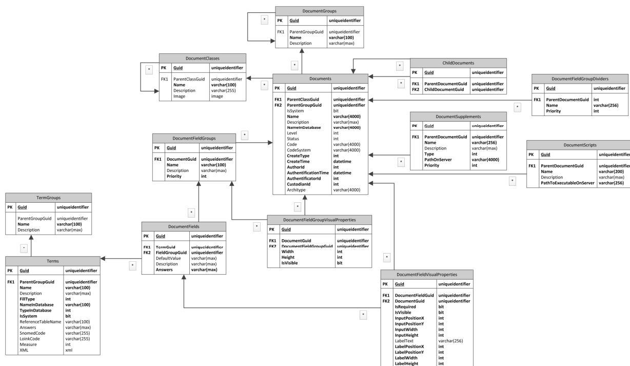
Figure 1. The open UMS BD structure
